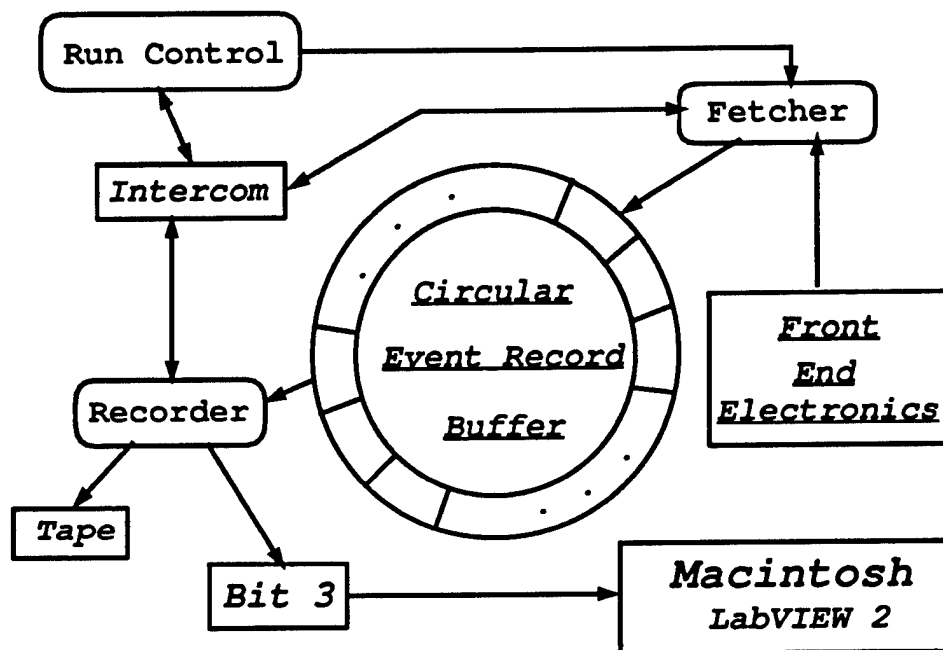
Figure II.C.7.2: The software logic for the RD93 DAQ system
