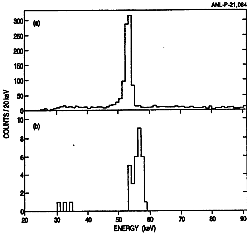
Figure II.B.3.1: Proton spectra of ^{147}\text{Tm} with time since recoil time a) between 10 ms and 5 s, and b) less than 10 ms.
