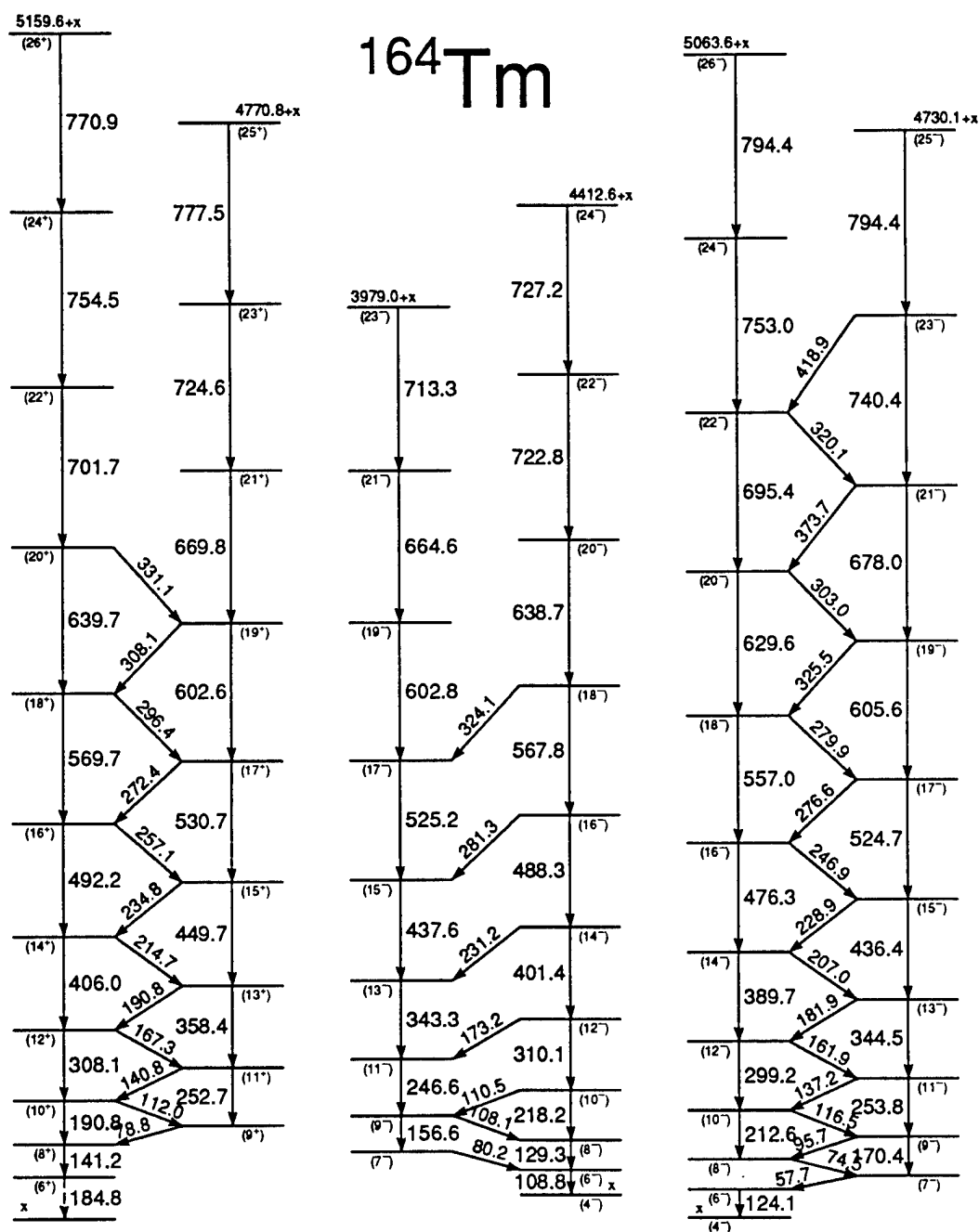
Figure II.A.6.1: Partial level scheme for ^{164}\text{Tm} . Spin and parity assignments to the bandheads are taken from Ref. [30]. Energy positions of the bandheads are unknown (labeled by x). The dashed 184.8 keV transition in the left band is uncertain. The placements of the new transitions in the scheme are based on the coincidence data from both the thin-target and backed-target measurements.
