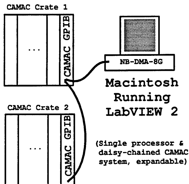
Figure II.C.6.1: Hardware layout for the small DAQ system.
