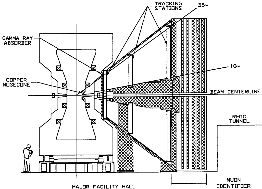
Figure II.C.2.1: Elevation view of PHENIX muon arm in the major facility hall.
