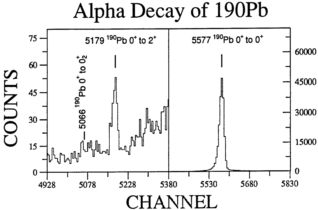
Figure II.B.1.1: Portion of the \alpha spectrum taken at the first counting station for the first four minutes after collection.
