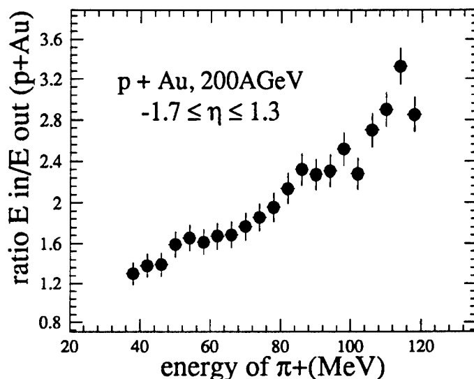
Figure II.C.10.2: Ratio of the pion kinetic energy spectra in-plane to out-of-plane in min. bias p + Au interactions at 200 GeV.
