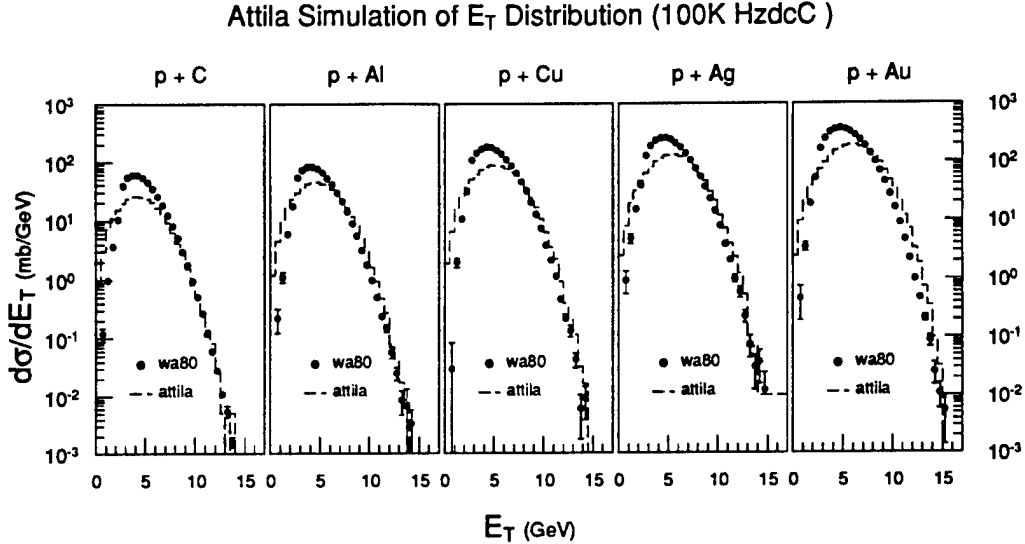
Figure II.C.9.1: Transverse energy spectra for 200 GeV proton induced reactions on ^{12}\text{C} , ^{27}\text{Al} , ^{nat}\text{Cu} , ^{nat}\text{Ag} , and ^{197}\text{Au} . The full circle points are from our measurement, the histograms from Attila simulation.
