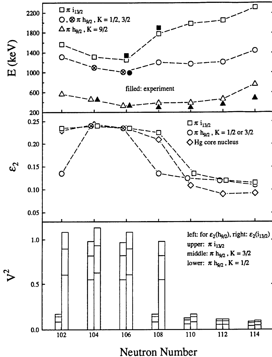
Figure II.A.1.2: Upper panel: Calculated bandhead energies for \pi i_{13/2} K = 1/2 (squares), \pi h_{9/2} K = 1/2 or 3/2 (circles) and \pi h_{9/2} K = 9/2 configurations (triangles) in odd-A Tl isotopes compared with experimental energies from this work, Ref. [4] and Ref. [11]. Middle panel: Calculated quadrupole deformations for the same cases and for Hg isotones. Lower panel: Occupation probabilities for low- K proton configurations in the respective Hg cores at two different \epsilon_2 values (left and right bin). Note that all calculations correspond to zero rotational frequency.
