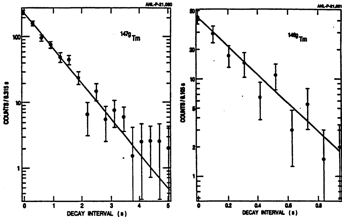
Figure II.B.3.2: Decay curves for ^{147g}\text{Tm} and ^{146g}\text{Tm} .
