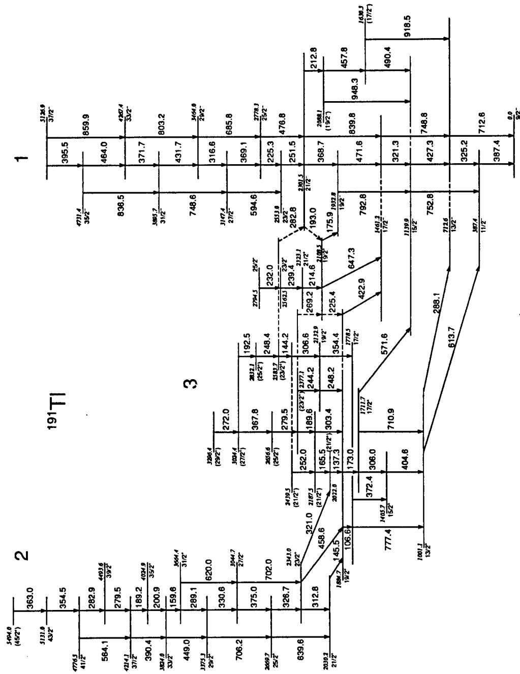
Figure II.A3.1: Level scheme for ^{191}\text{Tl} . Spin and parity assignments given in parentheses are tentative.
