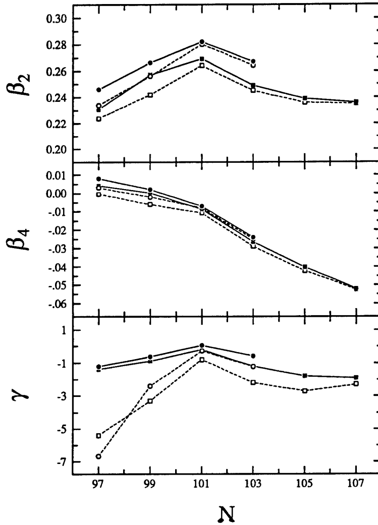
Figure II.A.8.1: Deformation parameters at \hbar\omega = 0.2 MeV for the \nu i_{13/2} bands in odd- A W nuclei. These values were extracted from TRS calculations. The open symbols refer to the favored signature ( \alpha = \frac{1}{2} ), and the filled symbols to the unfavored signature ( \alpha = -\frac{1}{2} ). The values for the Yb mesh are denoted by circles, the Pt mesh by squares.
