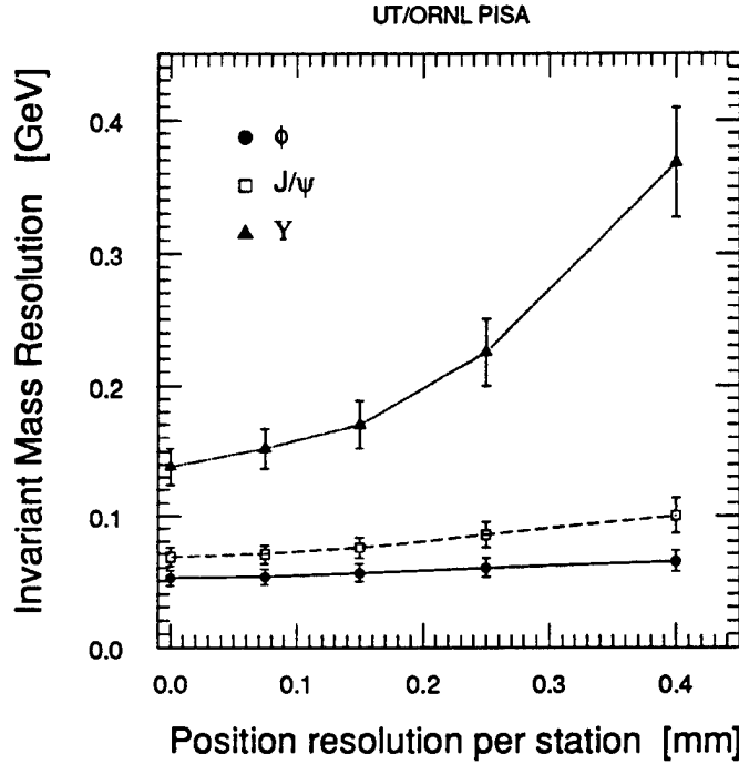
Figure II.C.2.3: Invariant mass resolution of dimuons originating from \phi , J/\psi and Y -decay as a function of the position resolution in the spectrometer tracking stations.
