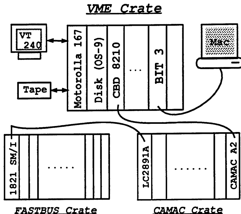
Figure II.C.7.1: The hardware layout for the RD93 DAQ system
