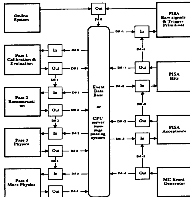
Figure II.C.3.2: Conceptual layout of the main modules of the event handling package and the simulation package. The data flow through the simulation system will be going from the event generator module at the lower right up to the digitization module in the upper right corner. The output from this module and the on-line system will be accepted by the off-line system for calibration, event reconstruction and data analysis. The main modules will exchange information through a set of data structures (labeled DS). This design will provide a high degree of modularity.
