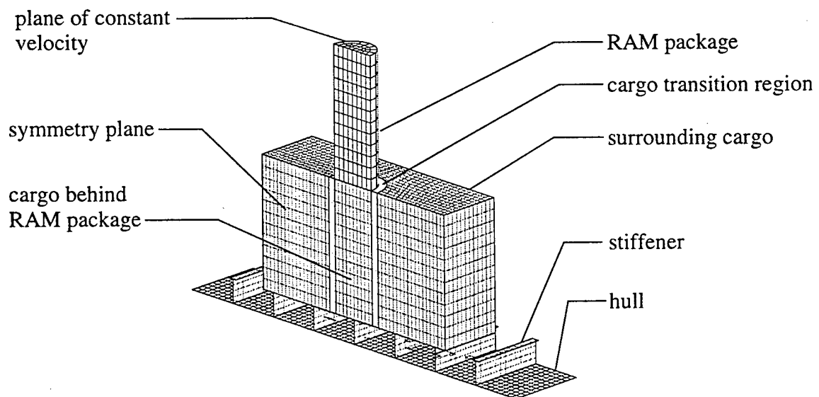
Figure 1: Schematic of the Finite Element Model
