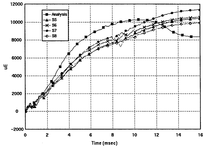
Strains at 12.7 cm from the center of the punch.
