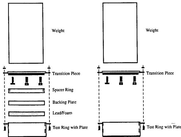
Figure 1: Schematic of test fixture configurations.
