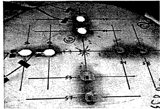
Figure 2: Strain gage placement on test units.
