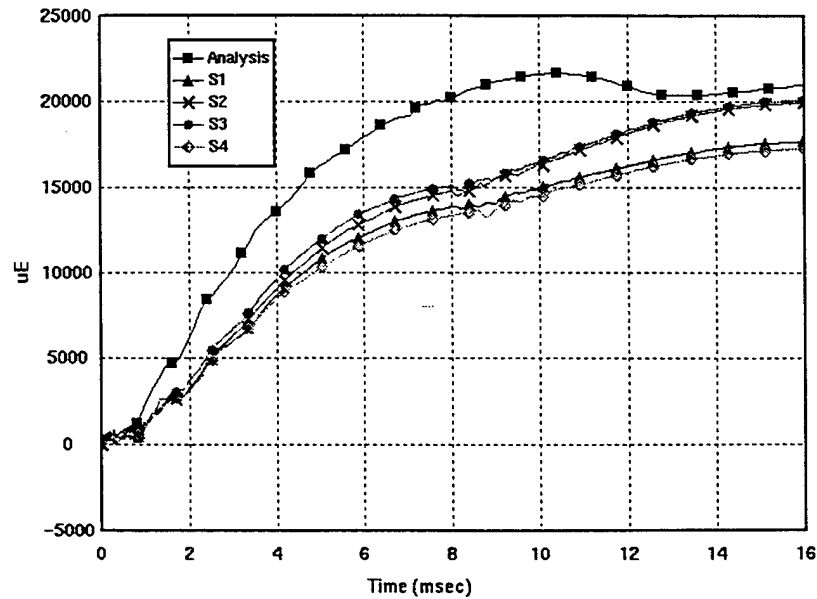
Strains at 7.6 cm from the center of the punch.
