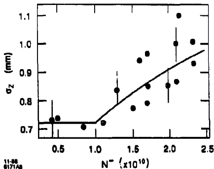
Fig. 6. Bunch length measurements versus N^- .
