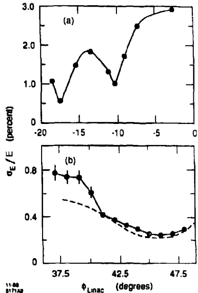
Fig. 9. Measured energy spectra of 47 GeV beams as a function of the linac overall RF phase. The measurement (a) is contaminated by anomalous dispersion in the linac which changes phase with the linac RF phase (because of energy). The measurement (b) has the anomalous dispersion in the linac removed and is close to the theoretical value.
