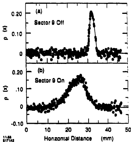
Fig. 5. Typical bunch width measurements with the spectrometer in Fig. 4 when the energy expander was turned off (a) and on (b). The bunch length measured in this example is 0.9 mm.
