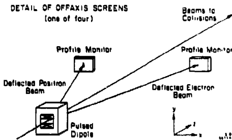
Fig. 12. Schematic of one of the four kicker-profile monitor combinations which allow both beams to be measured on a single linac pulse.
