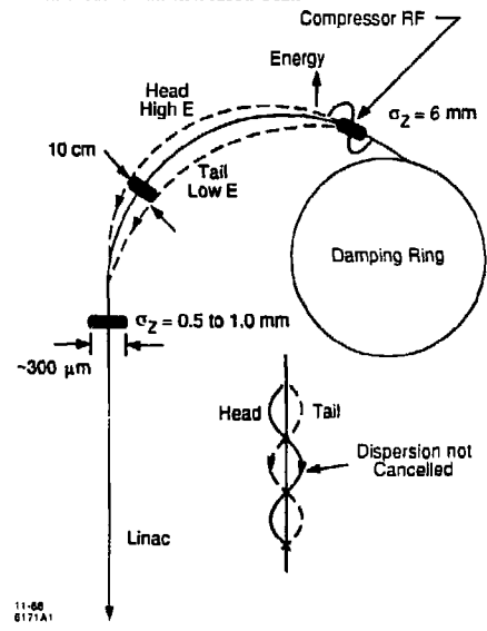
Fig. 1 After exiting the damping ring, each bunch is longitudinally compressed in the RTL transport line using an RF accelerator or compressor. The beam energy is 1.15 GeV, and the RF compressor provides a maximum of 92 MeV acceleration. The bunch center passes at the RF zero crossing. The energy dispersion \eta in the RTL must be cancelled to about one millimeter as the beam enters the linac or else there will be anomalous dispersion which will enlarge the effective beam emittance.
