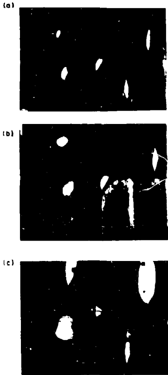
Fig. 13. Digitized "four" screen profile data for electrons using the equipment in Figs. 11 and 12. Photo (a) shows nominal beam profiles. Photo (b) shows enlargement of the beam due to betatron mismatches. Photo (c) shows enlargement of the beam due to a large anomalous dispersion in the linac.
