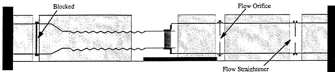
Figure A7.4 Leakage Flow Measurement Setup
