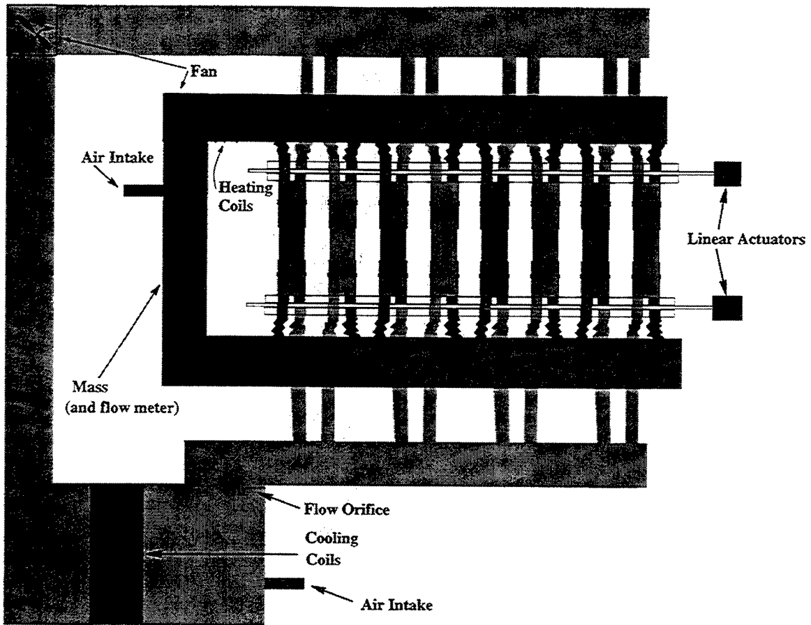
Figure A7.2 Longevity Test Apparatus
