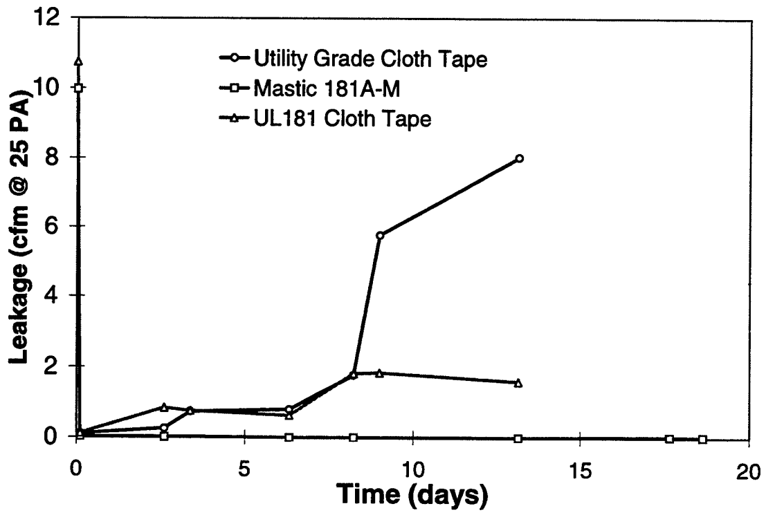
Figure 3. Changing test sample leakage from longevity test apparatus
