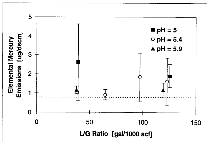
Figure 5.18 Impact of Scrubber Operating Conditions on Elemental Emissions - Open Tower
