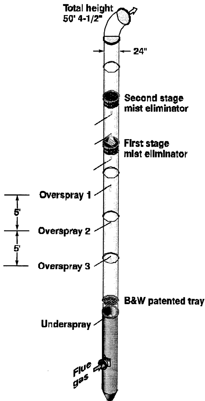
Figure 3.3 Wet Scrubber
