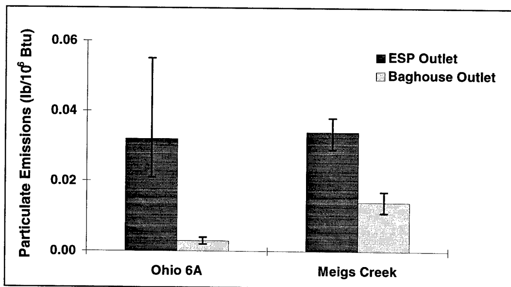
Figure 6.8 Particulate Emissions from ESP and Baghouse
