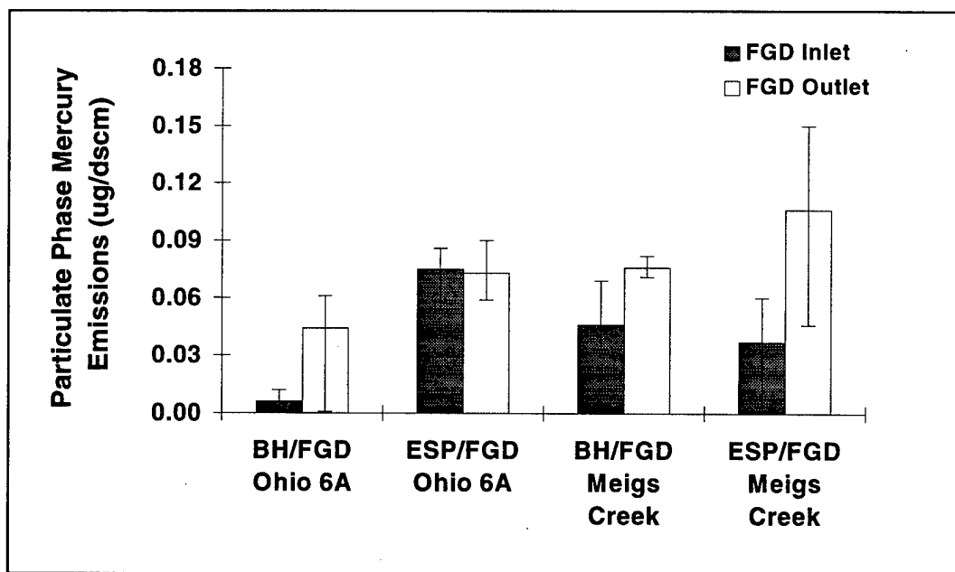
Figure 6.20 Particulate-Phase Mercury
