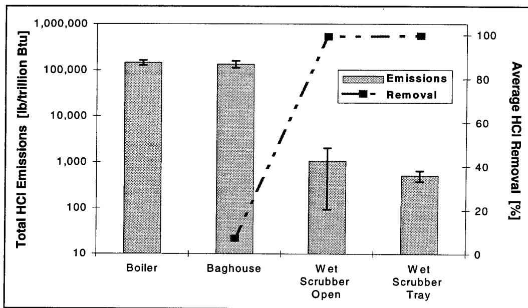
Figure 5.23 Hydrogen Chloride Control Summary - Test II
