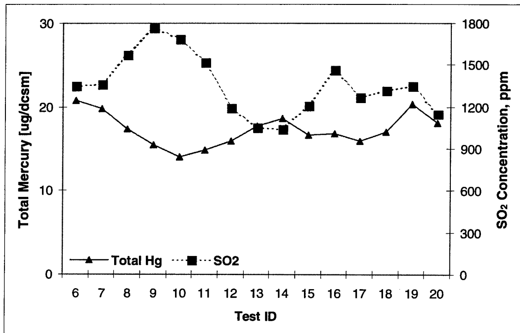
Figure 5.24 Comparison of \text{SO}_2 and Total Hg Concentrations - Burner 1
