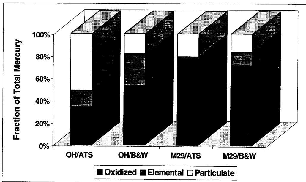
Figure 4.22 Uncontrolled Mercury Speciation Data: Ontario Hydro and Method 29
