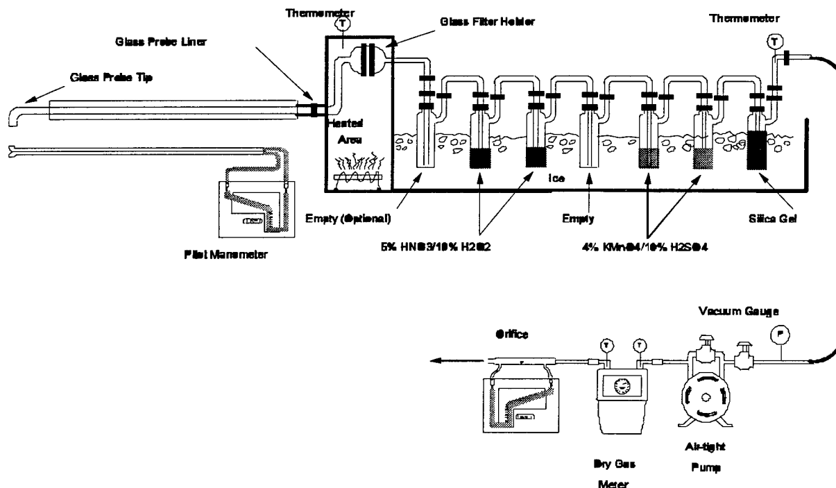
Figure 4.2 Method 29 Sampling Train
