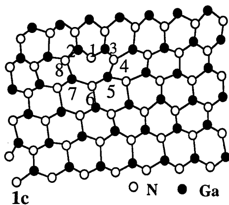
Fig.1(a) High-resolution Z-contrast image of a threading edge dislocation looking down \langle 0001 \rangle . (b) Maximum entropy image of (a) showing most probable column positions. (c) Sketch of the core structure determined from the experimental data.
