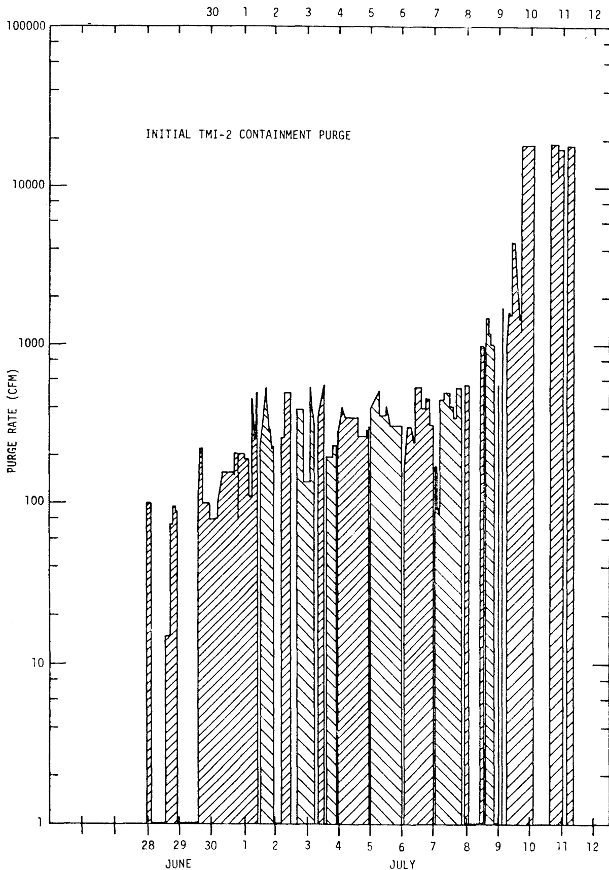
Figure 3. Histogram of Venting Rates June 28 to July 11, 1980
