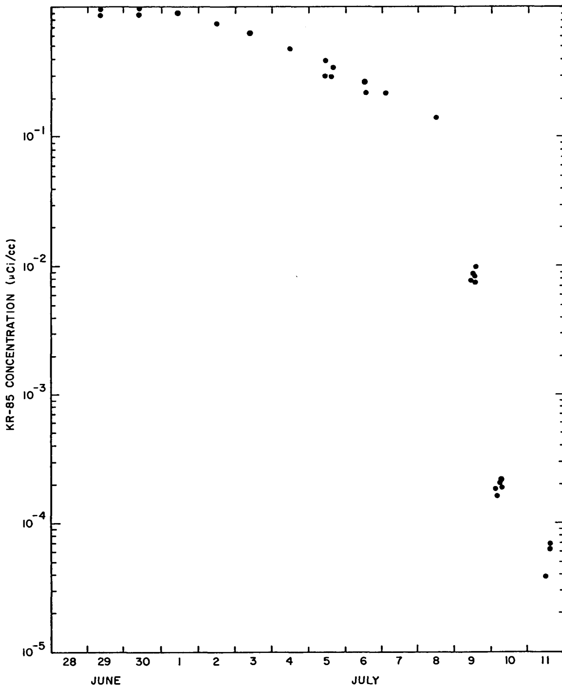
Figure 4 Reactor Building Atmosphere, Kr-85 Samples.
