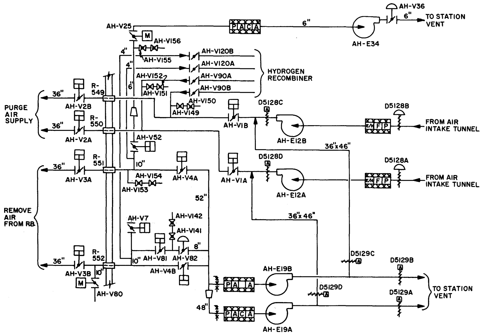
Figure 1 TMI-2 Purge System.
