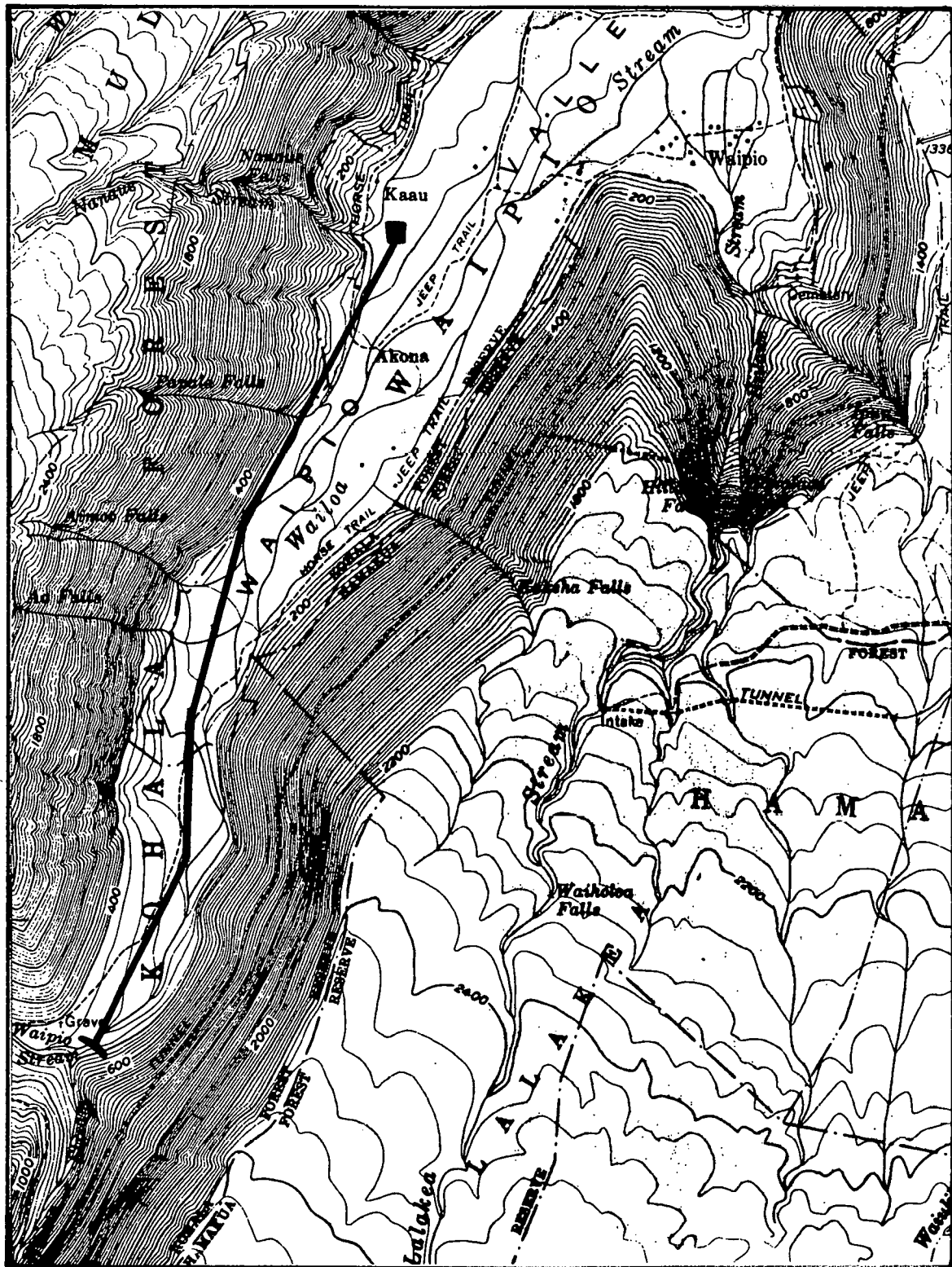
Figure D-52. Prospective Hydropower Site, Waipio River, Hawaii.
