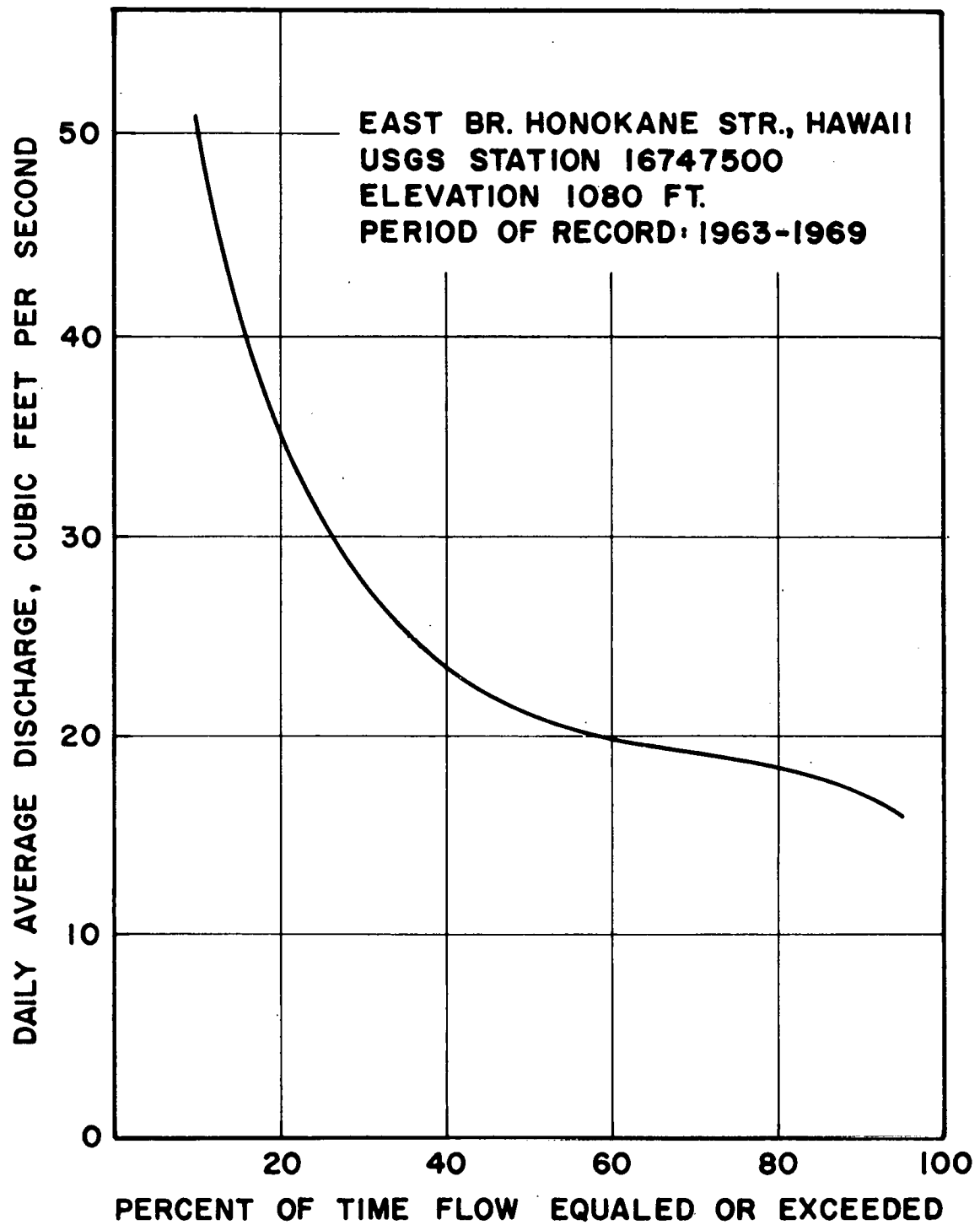
Figure D-59. Flow Duration Curve, E. Br. Honokane Nui Stream, Hawaii. (Based on U.S.G.S. Water Resources Division Stream Gage Data)
