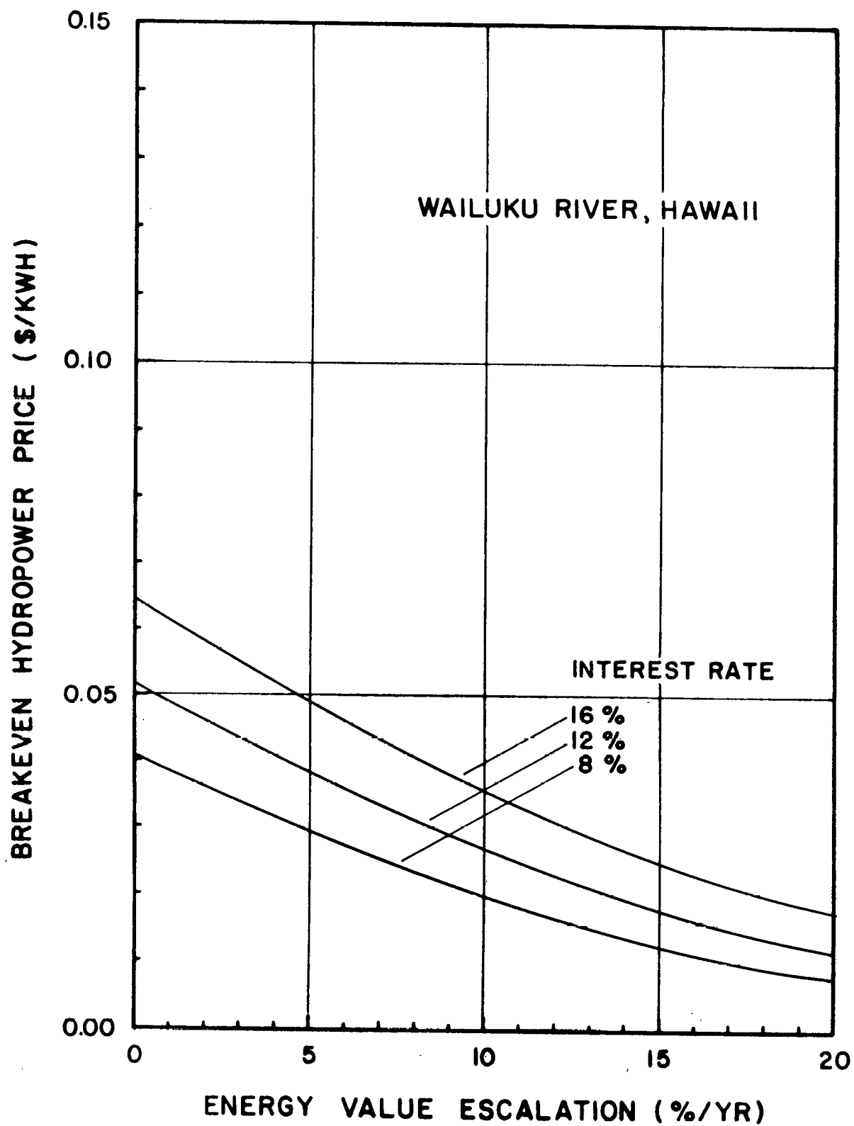
Figure D-51. Breakeven Hydropower Price as a Function of Interest Rate and Energy Value Escalation Rate, Wailuku River, Hawaii.
