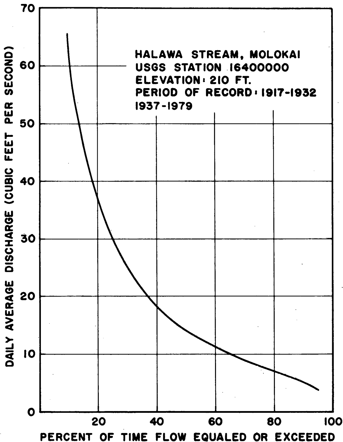
Figure D-20. Flow Duration Curve, Halawa Stream, Molokai. (Based on U.S.G.S. Water Resources Division Stream Gage Data) D-33
