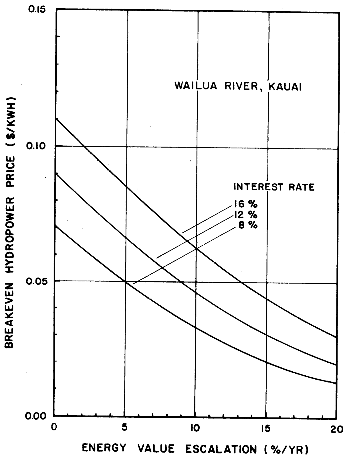
Figure D-2. Breakeven Hydropower Price as a Function of Interest Rate and Energy Value Escalation Rate, Wailua River, Kauai.
