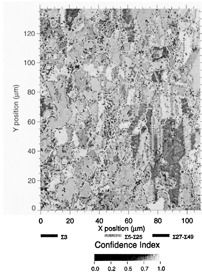
Figure 5. OIM image of the as recrystallized structure shaded by confidence index with special (grey shaded) and random (white) boundaries indicated.
