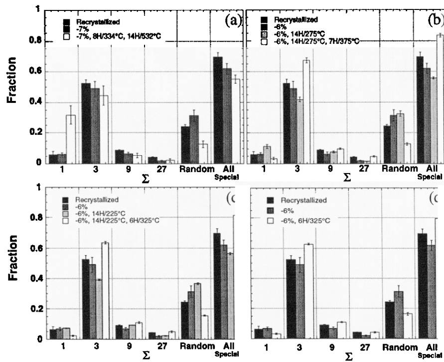
Figure 6. Fraction of boundaries of indicated type as a function of strain annealing treatment: (a) OFE-1, (b) OFE-2, (c) OFE-3, and (d) OFE-4.
