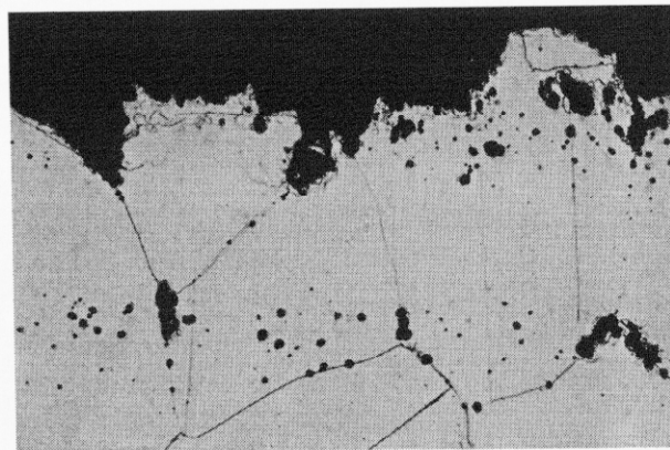
Figure 1. Optical micrograph showing the development of a spall plane in Cu. (5)
