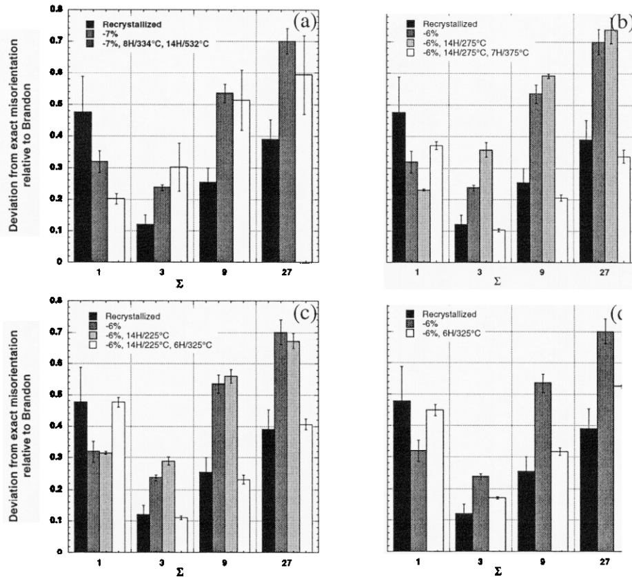
Figure 7. Deviation from exact misorientation plotted as a function of boundary type for each strain annealing treatment: (a) OFE-1, (b) OFE-2, (c) OFE-3, and (d) OFE-4.
