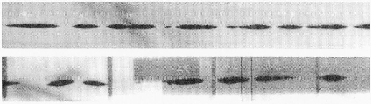
Figure 2. Radiographs of Cu shaped-charge jets. The jet at top is undoped OFE copper. The jet at the bottom was produced from Cu that had S segregated to the grain boundaries. The effect of the S is earlier breakup of the jet and formation of asymmetric particles. (6)
