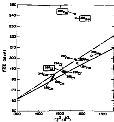
Fig. 4. Total kinetic energy vs. Z^2/A^{1/3} for SF of heavy actinide isotopes. The dashed line is the fit of Unik et al. 7 and the solid line is the fit of Viola et al. 8
