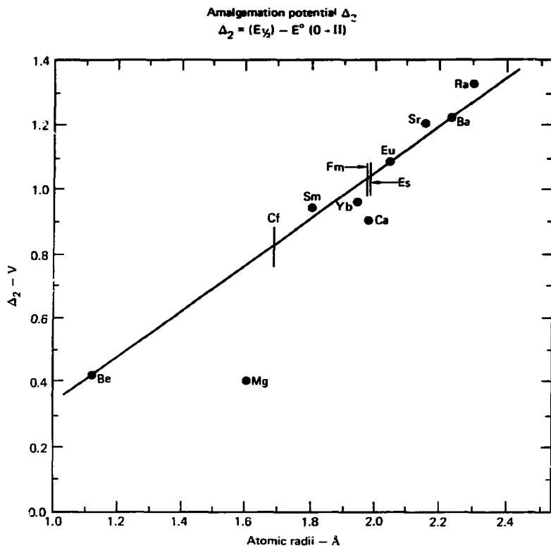
Fig. 3. Amalgamation potentials, \Delta_2 , derived from experimental data are plotted as a function of the atomic (metallic) radii. The amalgamation potential for Fm is obtained by using an estimated radius. (Partially redrawn from Ref. 10).
