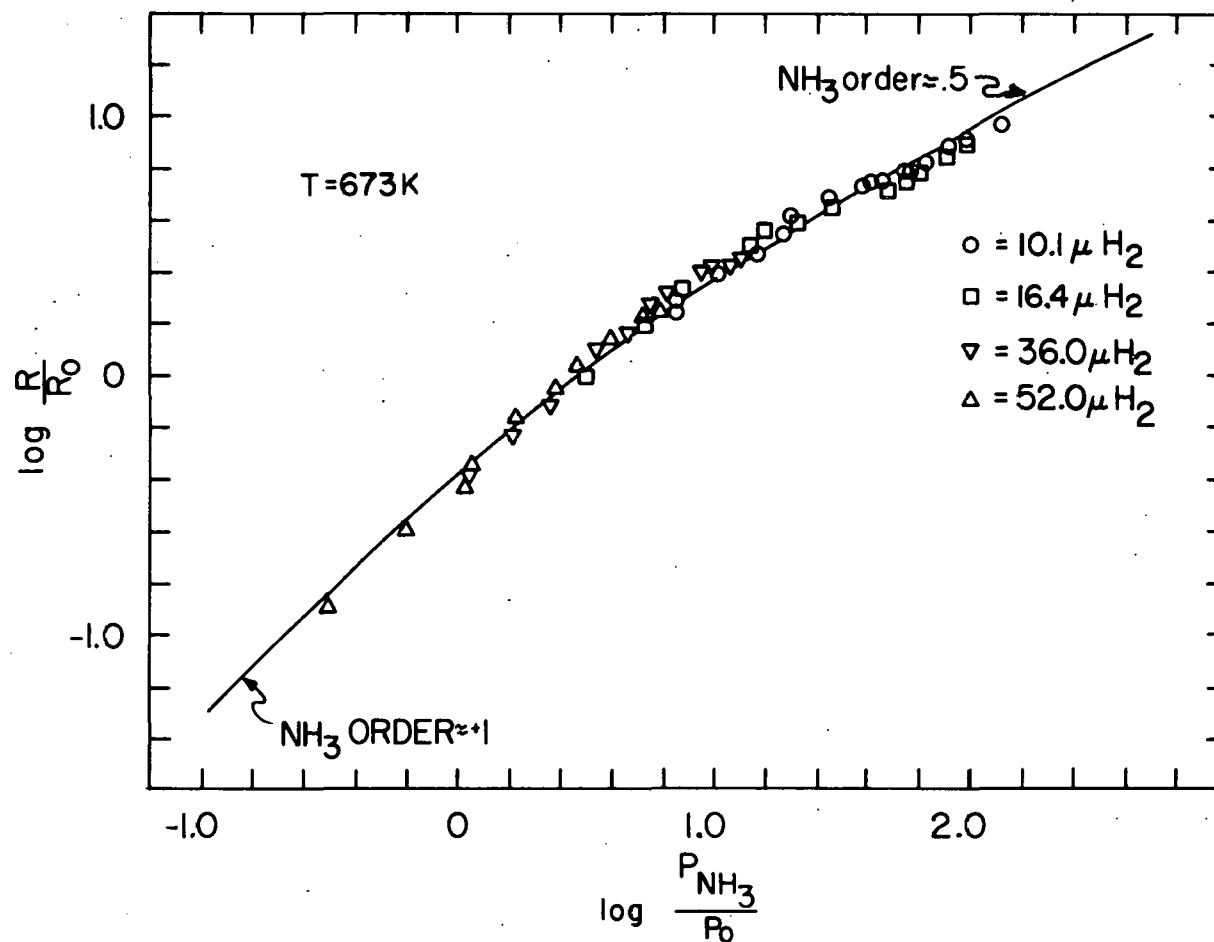
Figure I-16. Superposition of NH_3 order data at fixed P_{H_2} on log-log curve representing the function defined by equation I-17 at 673K (See Table I-2 for appropriate parameters.)
