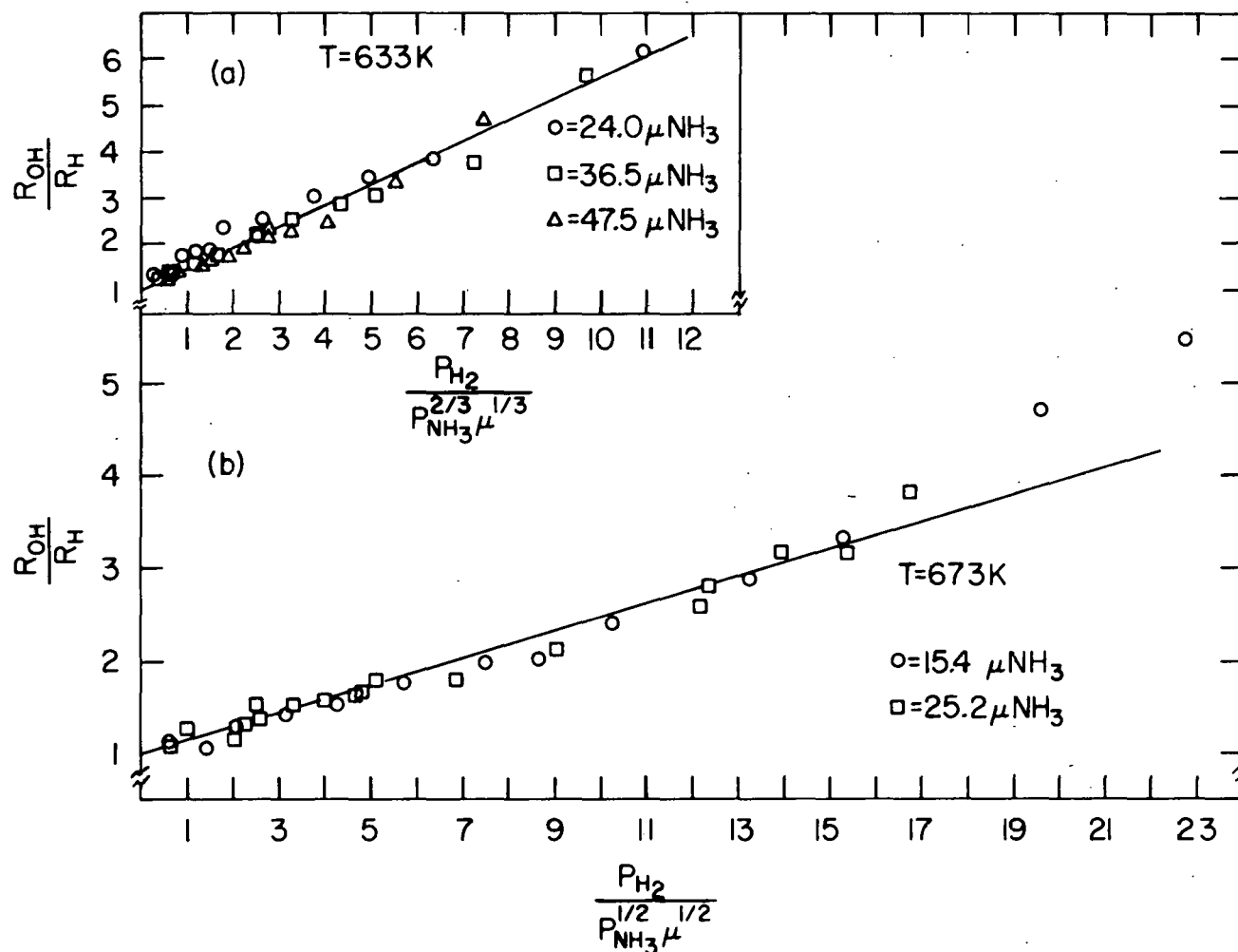
Figure I-21. Superposition of all H_2 order data on linear plots with slopes equalling k''' as defined in equation I-26: (a) 633K, k''' = .45 \mu^{-1/3} ( P_{H_2} = 54 \mu data omitted for clarity); (b) 673K, k''' = .147 \mu^{-1/2}
