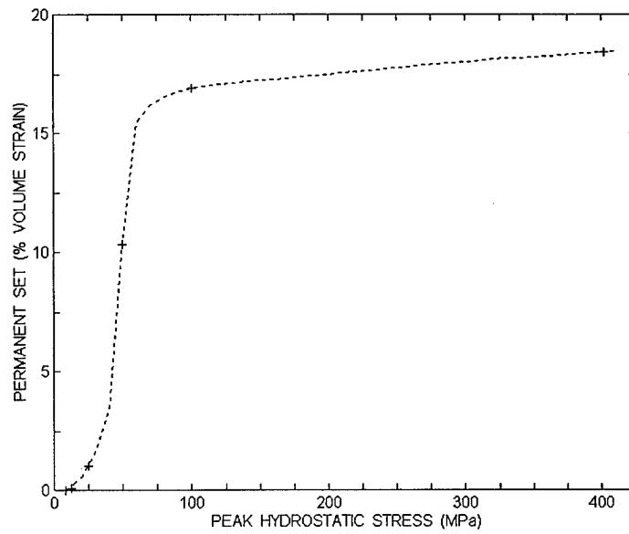
Fig. 10. Permanent set for shock conditioned HPNS-5 (R-1) grout as a function of peak hydrostatic stress. Data obtained from mechanical tests are indicated with '+' marker.
