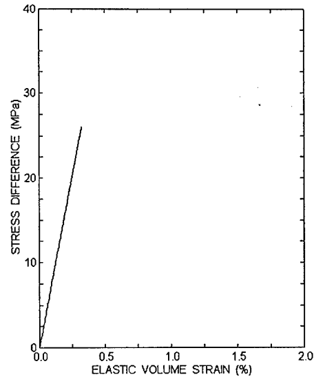
Fig. 15b. Elastic volume strain contribution to specimen 301 in triaxial compression.
