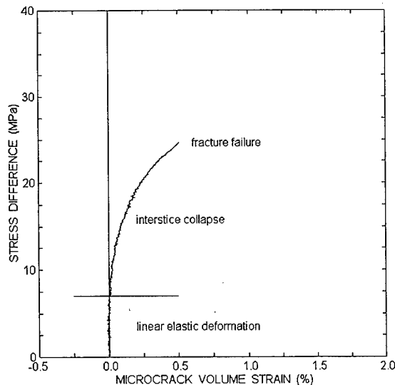
Fig. 14a. Deviation from linear elastic deformation for shock conditioned specimen HPNS5-DZ-DRM2#2 subjected to uniaxial compression.
