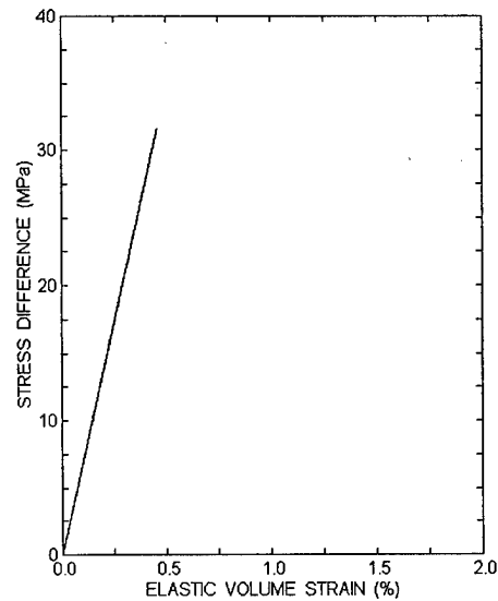
Fig. 13b. Elastic volume strain contribution to specimen HPNS5-U3 in uniaxial compression.
