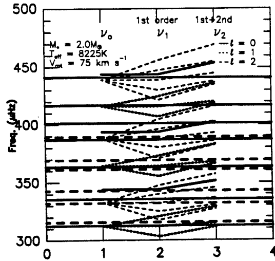
Figure 2. A schematic illustration of the importance of rotational splitting on the frequencies of CD-24° 7599. \nu_0 are frequencies without rotational splitting, \nu_1 includes first order rotation corrections, and \nu_2 includes both first and second-order corrections.
