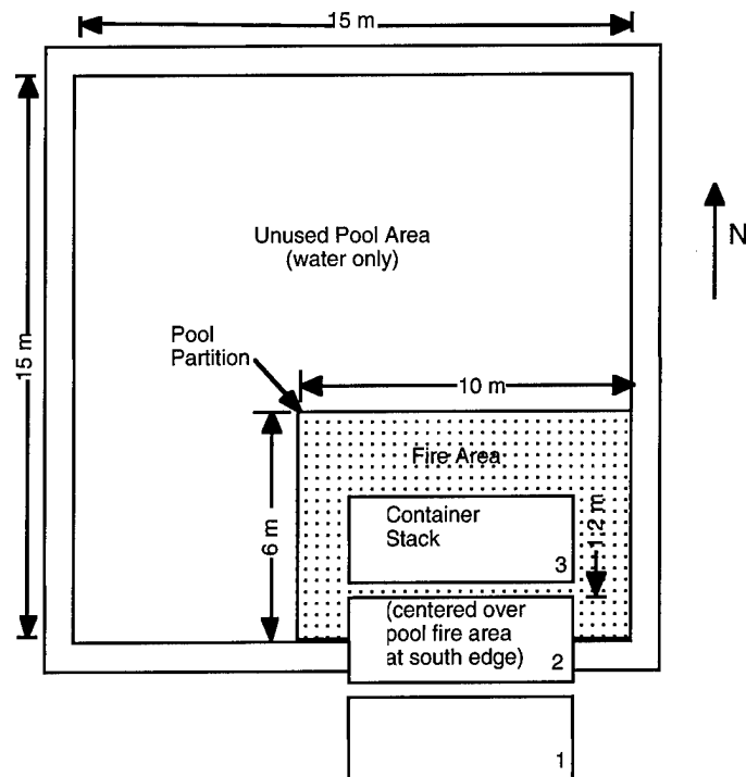
Figure 2. Plan view of fire test arrangement
