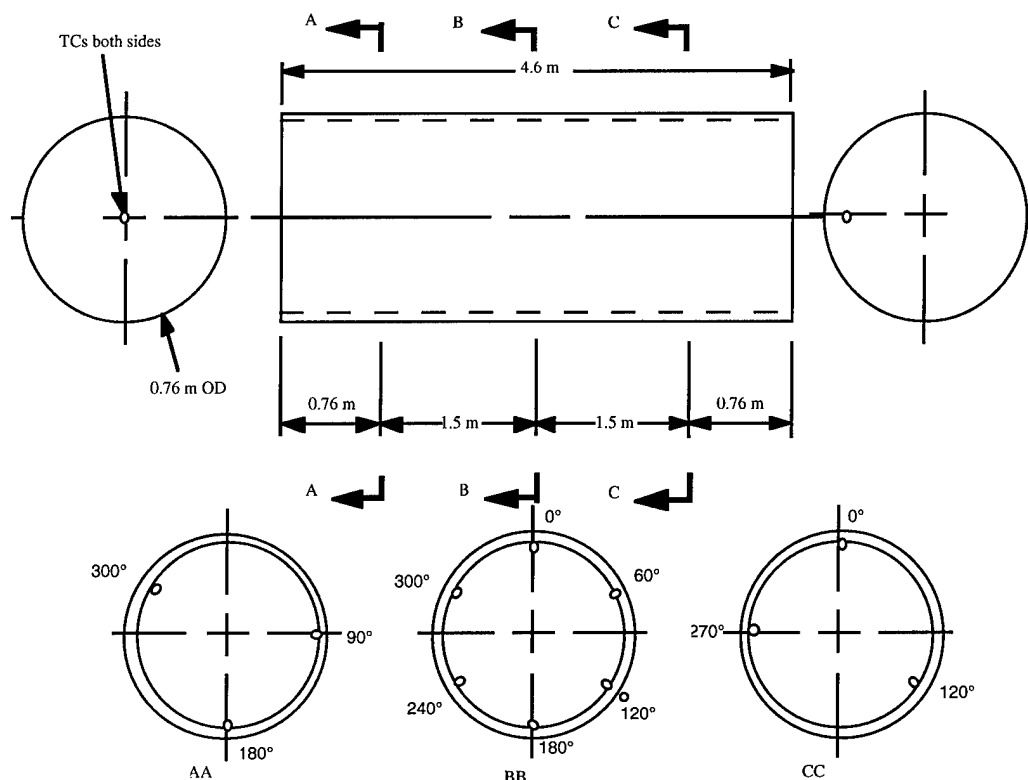
Figure 3. Thermocouple arrangement for large, stainless steel calorimeter.
