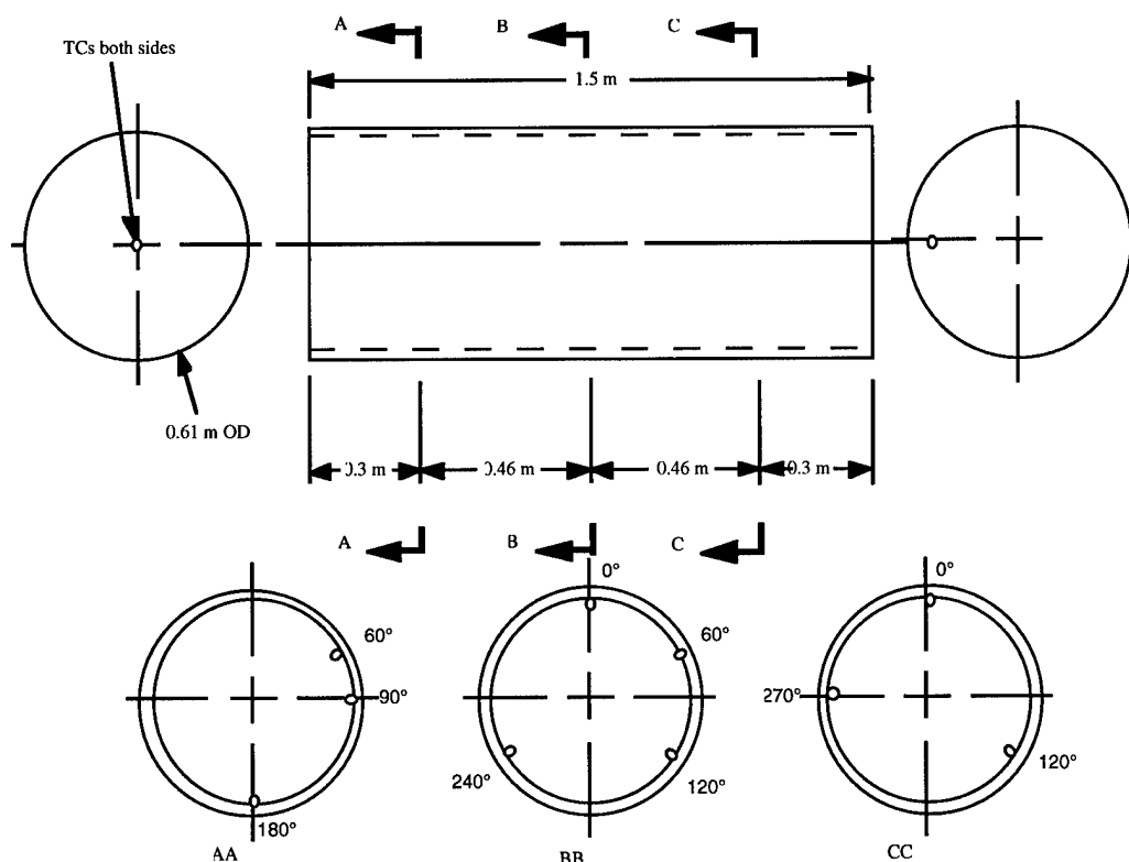
Figure 4. Thermocouple arrangement for carbon steel calorimeters.
