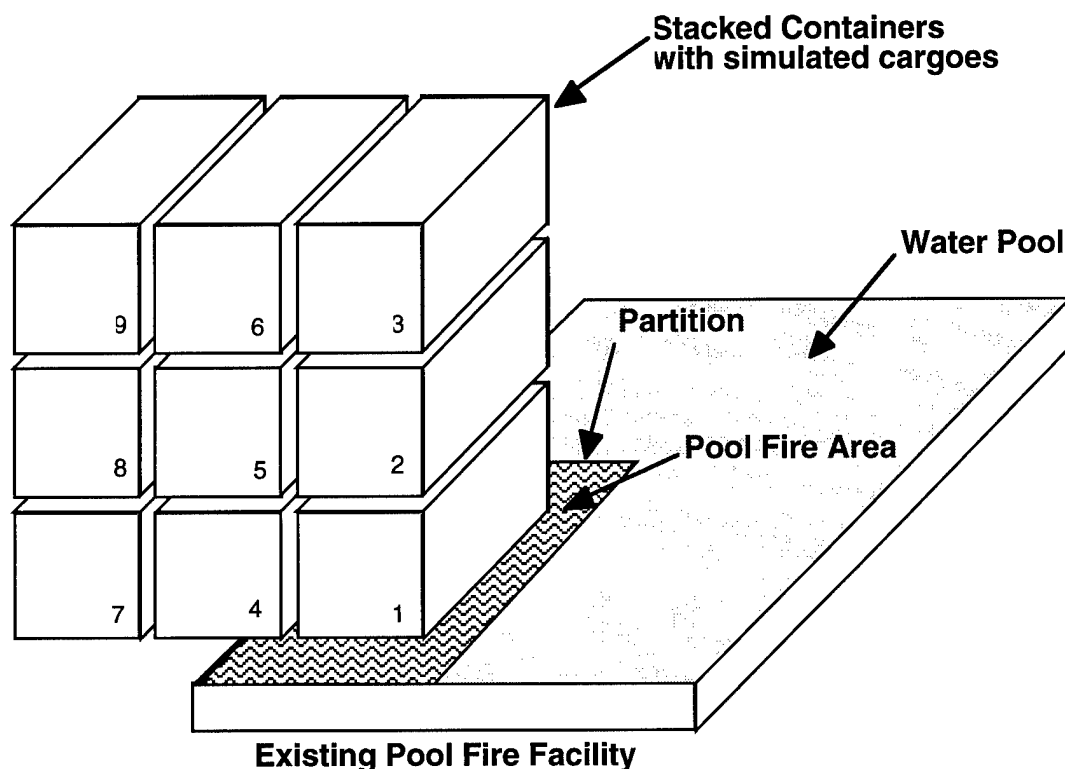
Figure 1. Schematic of fire test arrangement.
