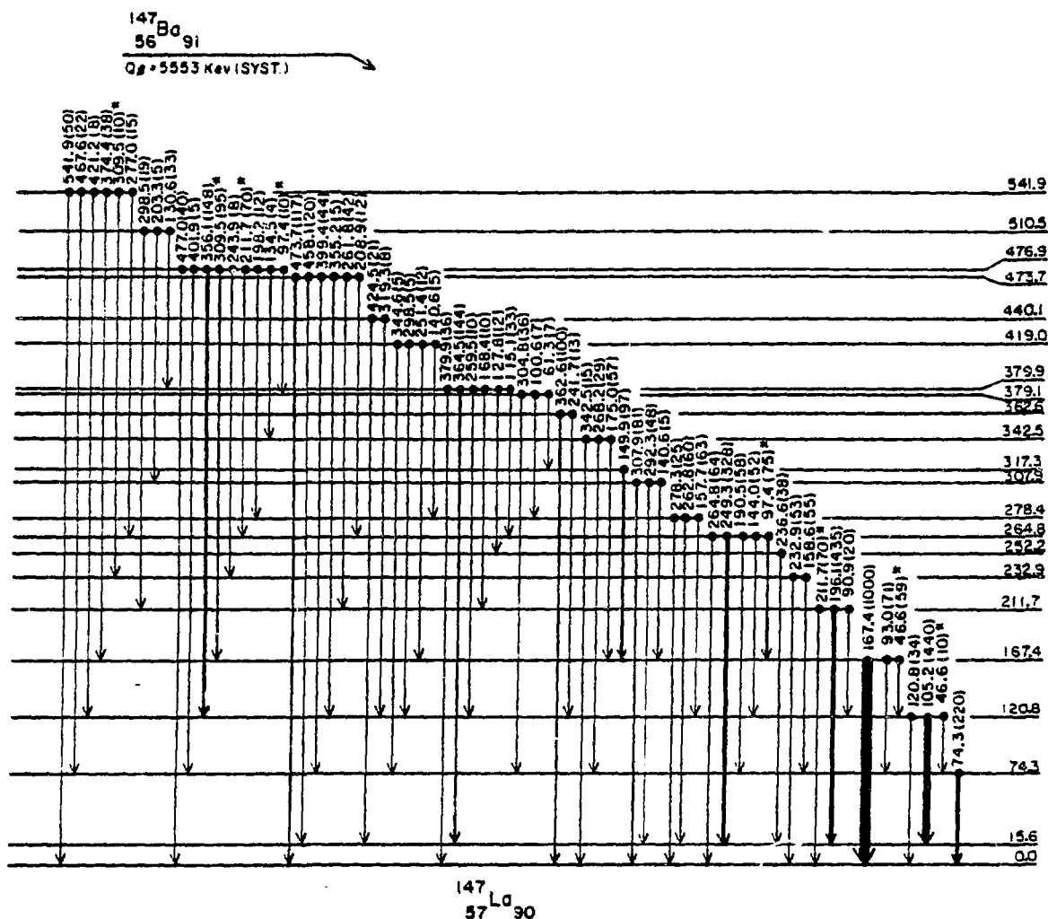
Fig. 1 A proposed decay scheme for ^{147}\text{Ba} ; levels up to 600 keV. *Multiple placement.
