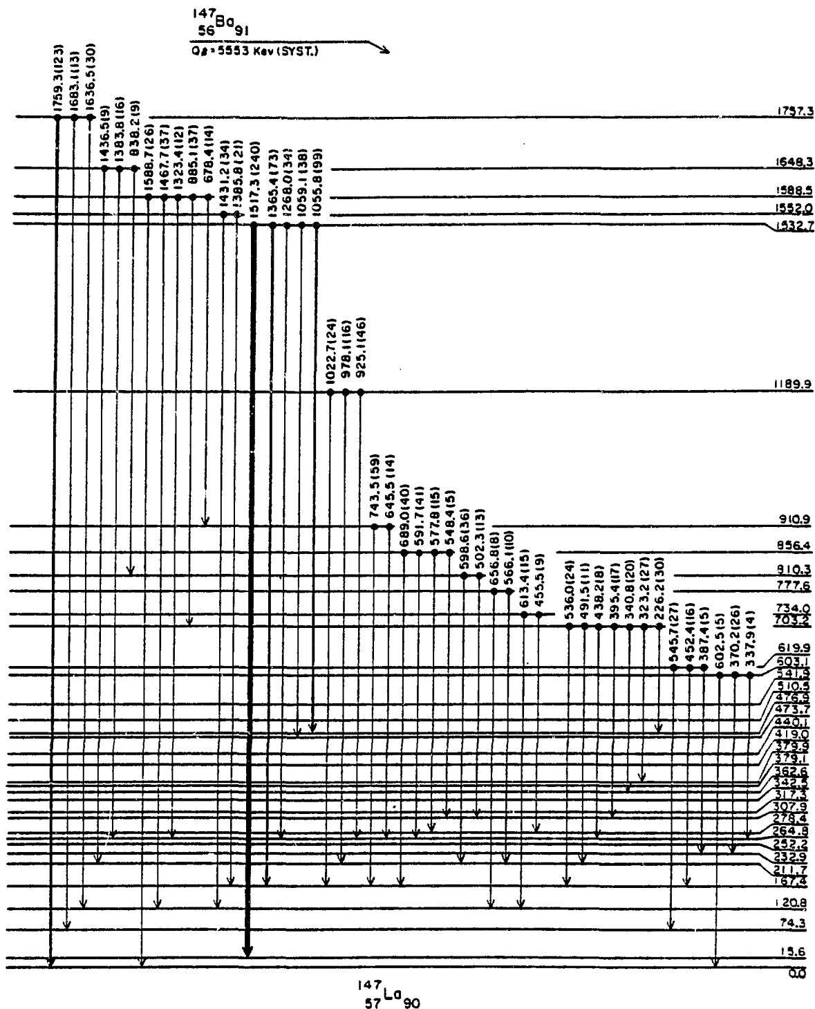
Fig. 2 A proposed decay scheme for ^{147}\text{Ba} : decay pattern of levels above 600 keV.
