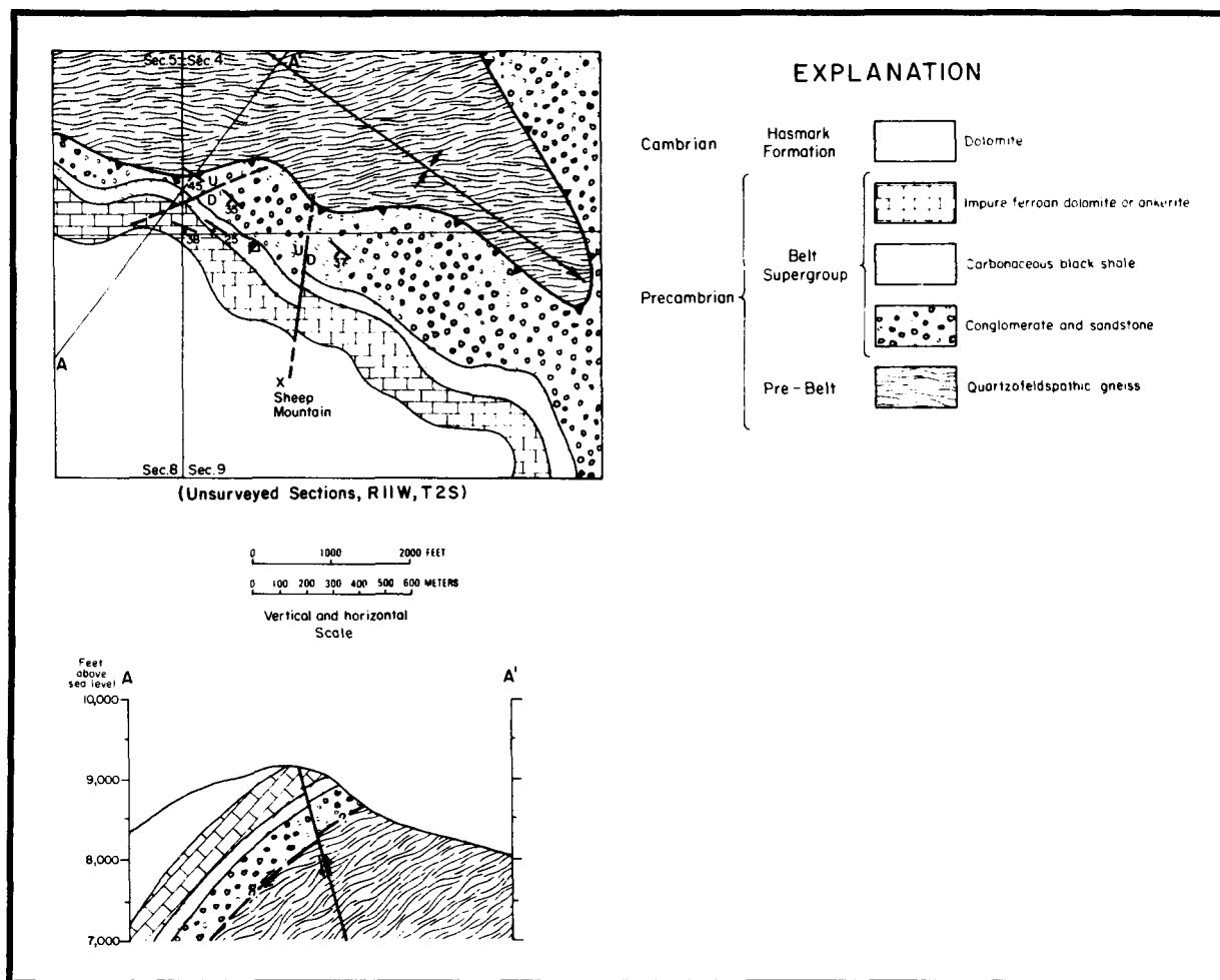
Figure 10. Geologic map and cross section of Sheep Mountain.
