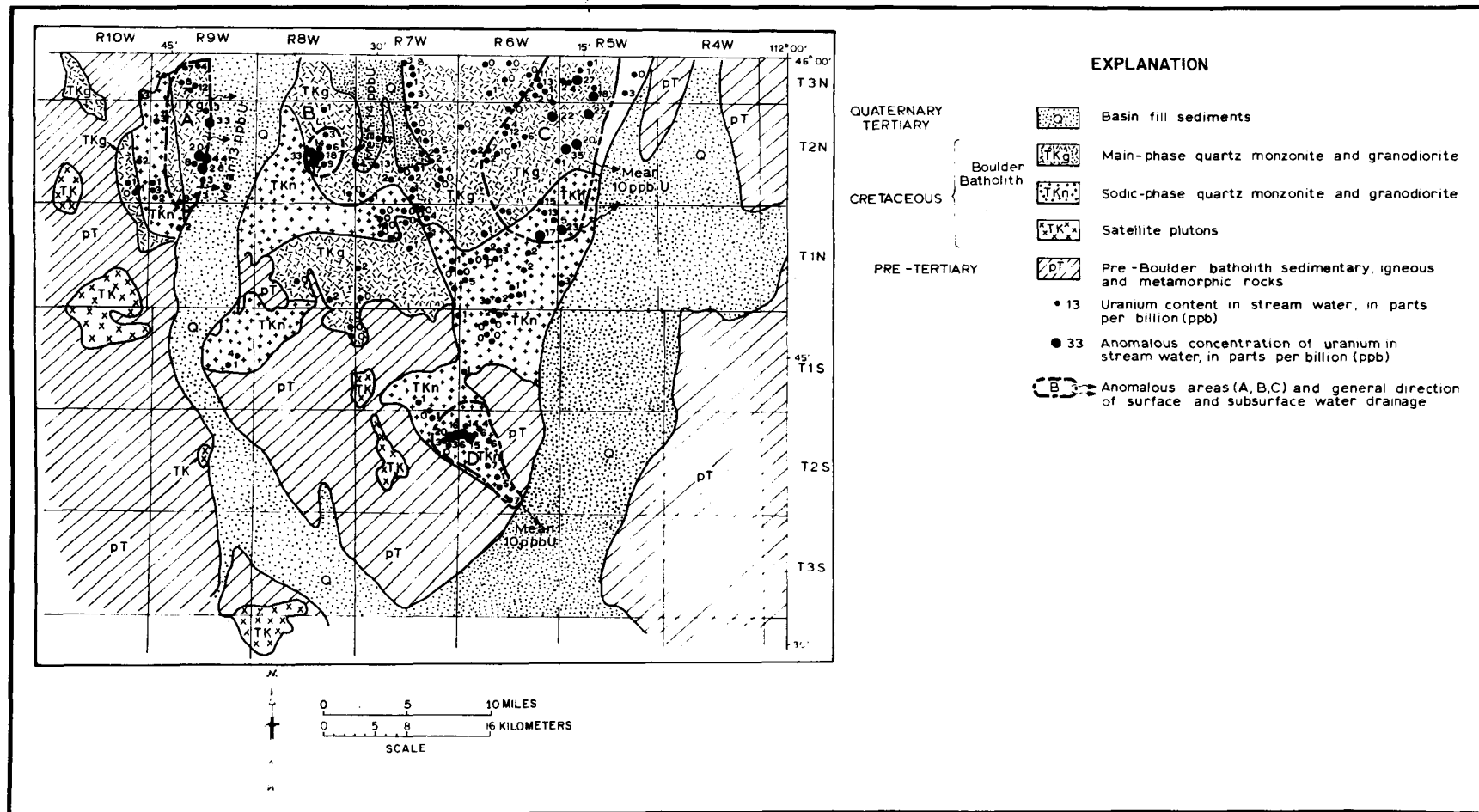
Figure 6. Sketch map of southern part of Boulder batholith showing sodic and main phases of quartz monzonite and granodiorite relationship of geochemical results in water including areas of anomalous amounts of uranium in stream waters.
