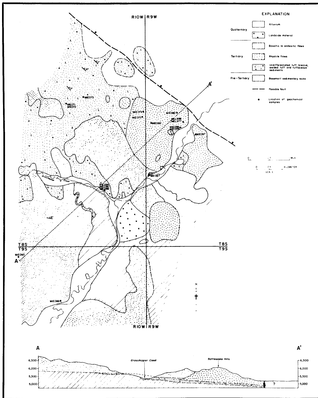
Figure 16. Geologic map and cross section of the Beaverhead River-Grasshopper Creek area, southwest of Dillon.
