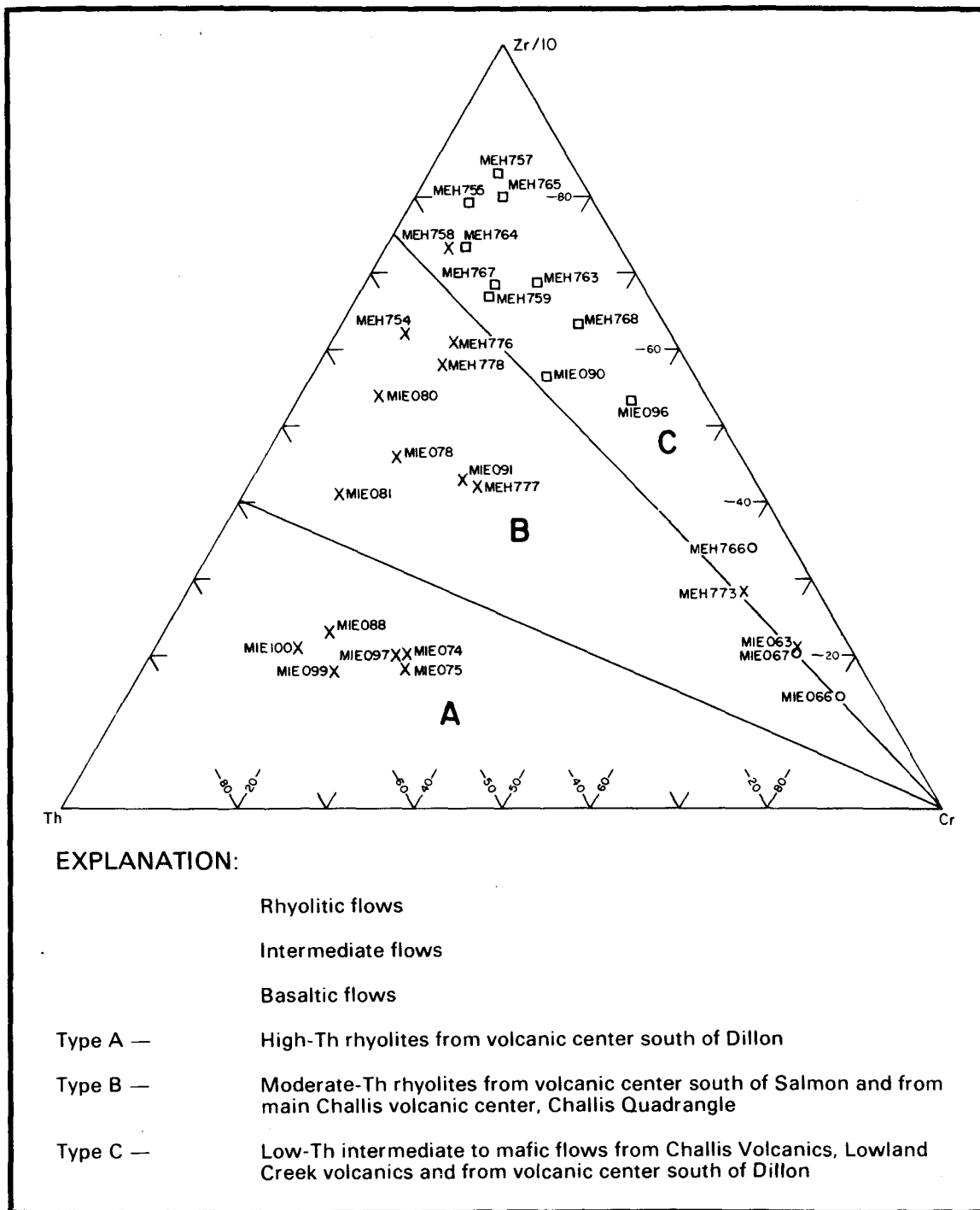
Figure 3. A ternary Zr-Th-Cr discrimination diagram for flow rocks from Dillon and Dubois Quadrangles.
