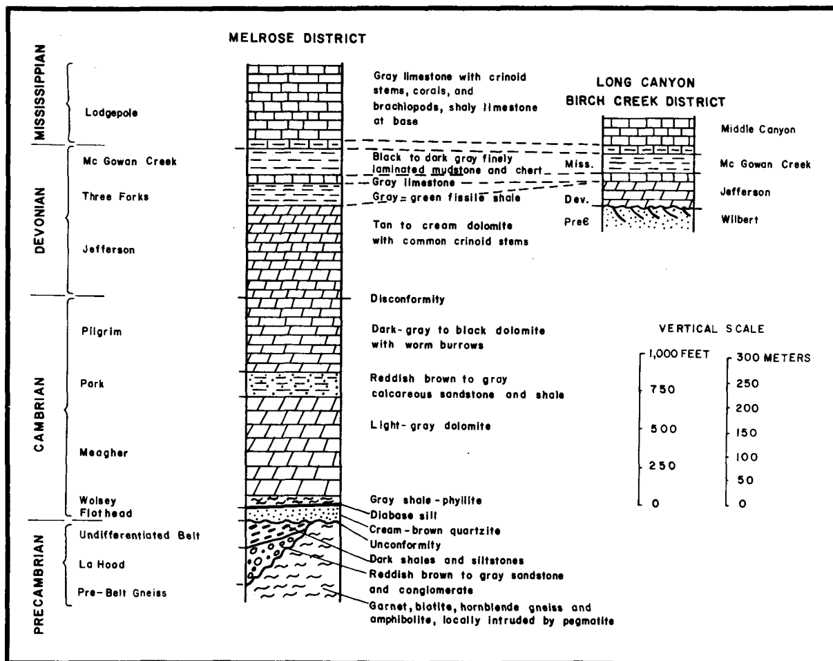
Figure 13. Stratigraphic column in the Melrose district with possible correlation in the Birch Creek district.
