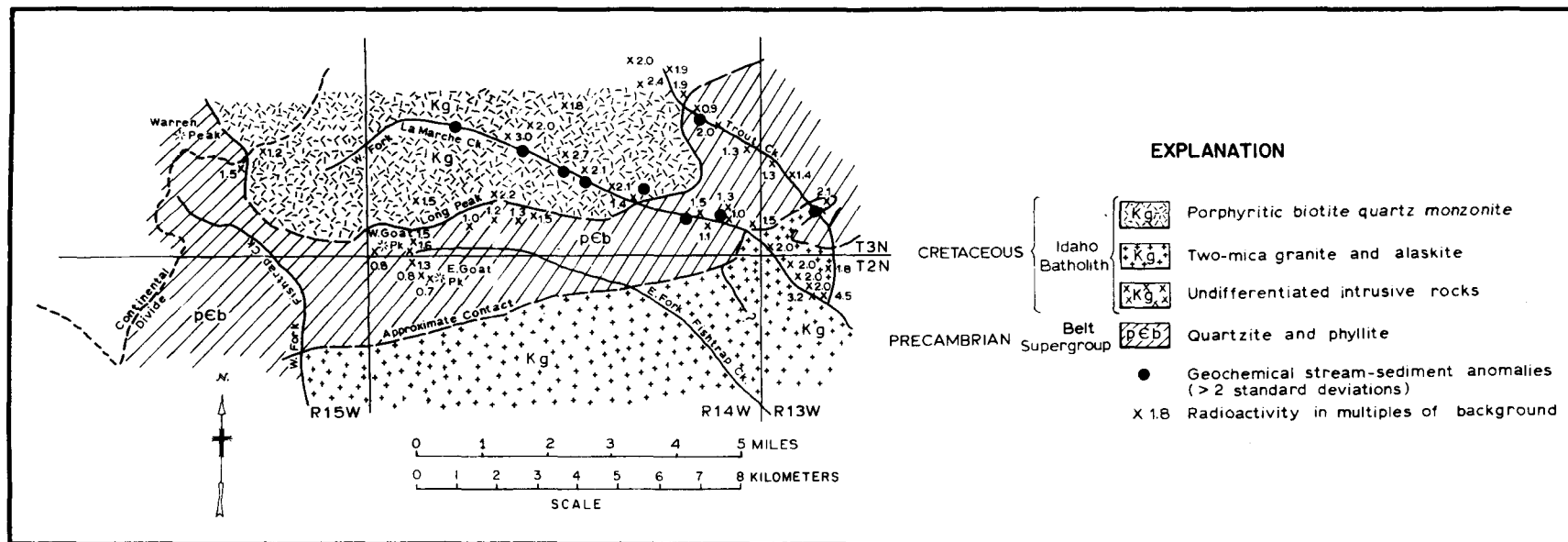
Figure 8. Geologic map and geochemical and radiometric sample locations, LaMarche Creek area, Anaconda-Pintlar Wilderness.
