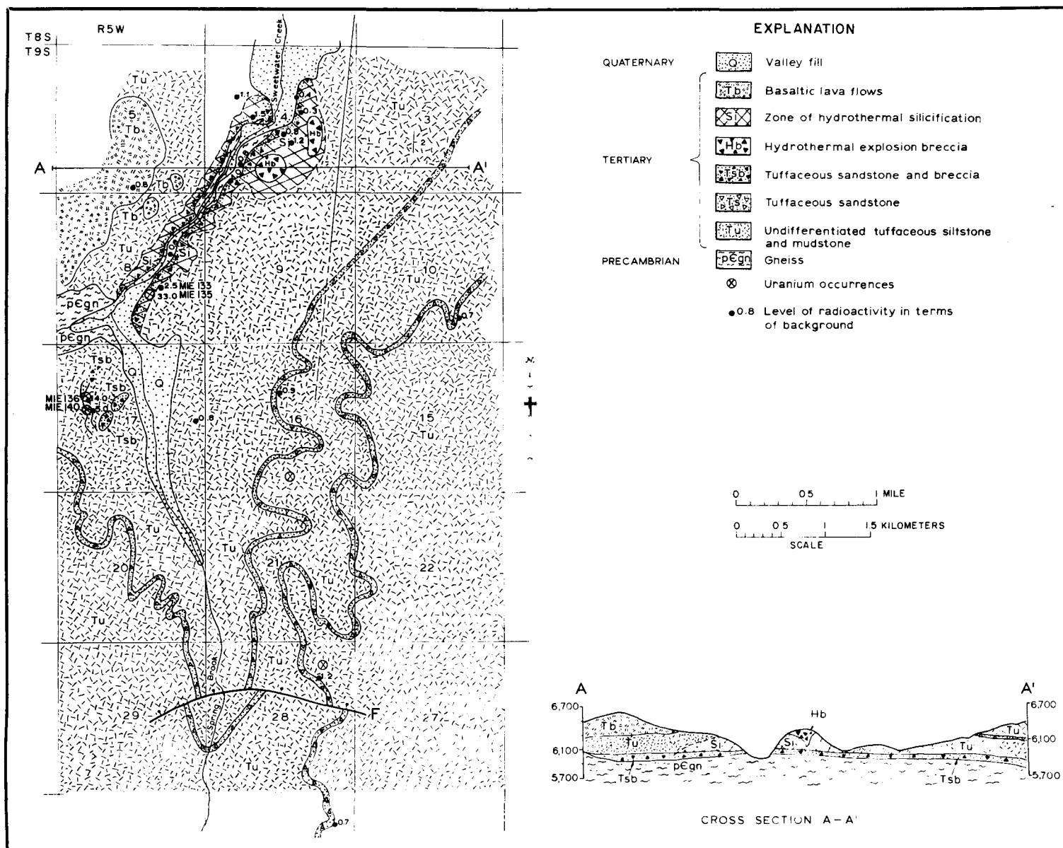
Figure 17. Geologic map and cross section of Sweetwater Creek-Spring Brook area.
