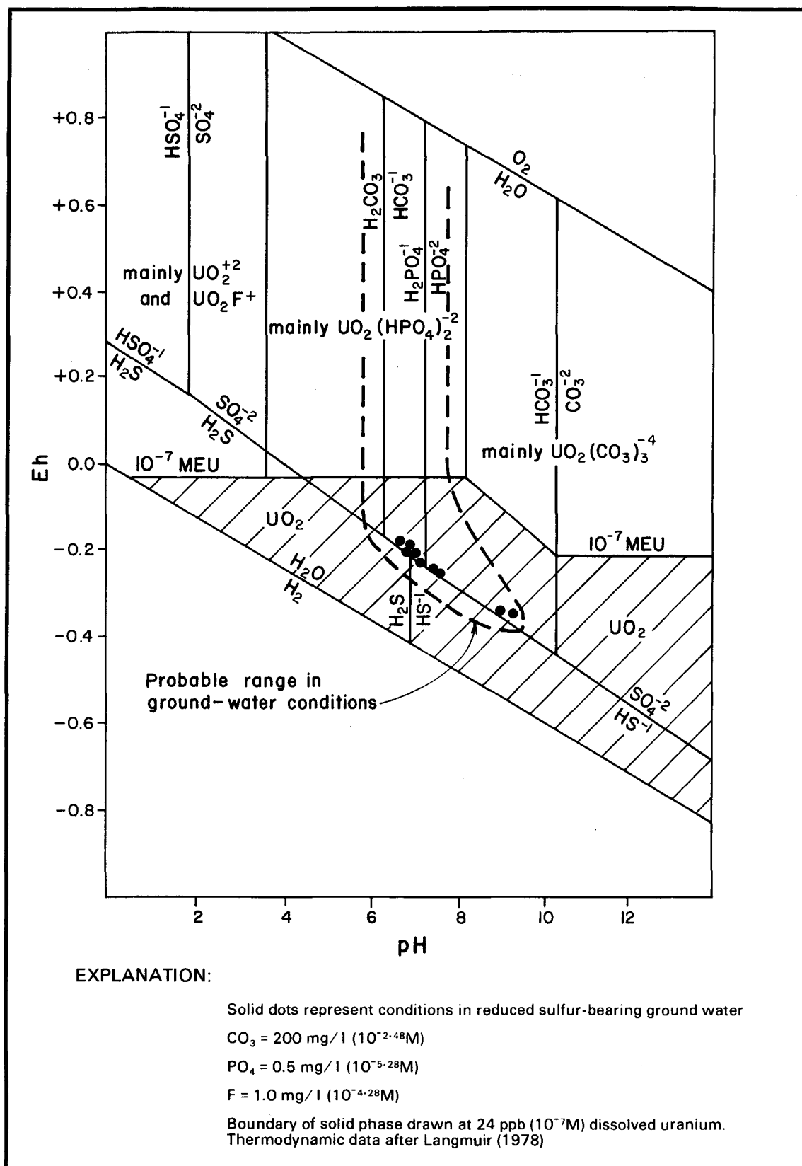
Figure 2. Partial aqueous equilibrium diagram of system U-O 2 -CO 2 -P-F-H 2 O, showing probable range of ground-water conditions.
