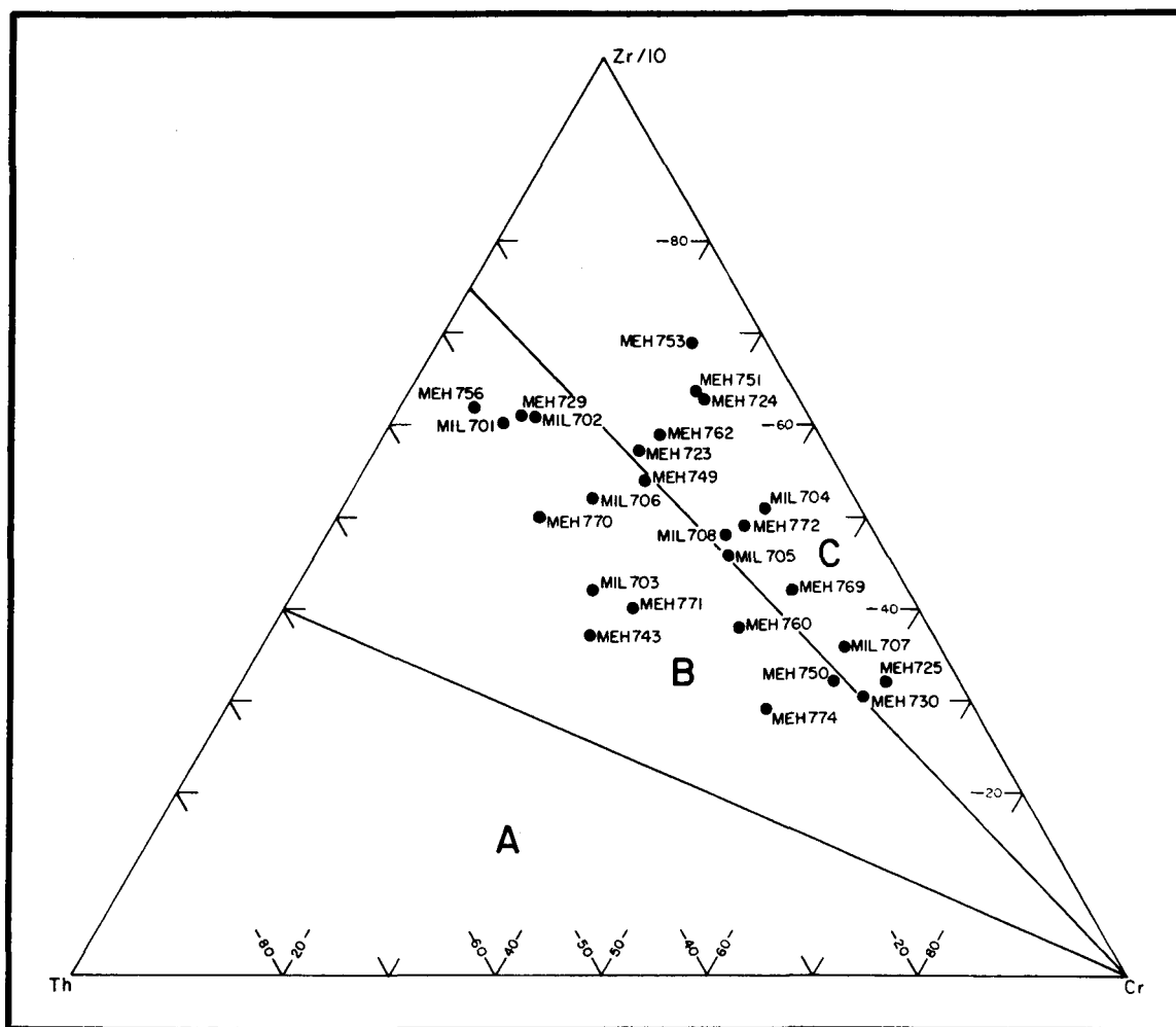
Figure 5. A ternary Zr-Th-Cr discrimination diagram for tuffs from Dubois Quadrangle. Areas A, B, and C drawn from discrimination diagram for flow rocks.
