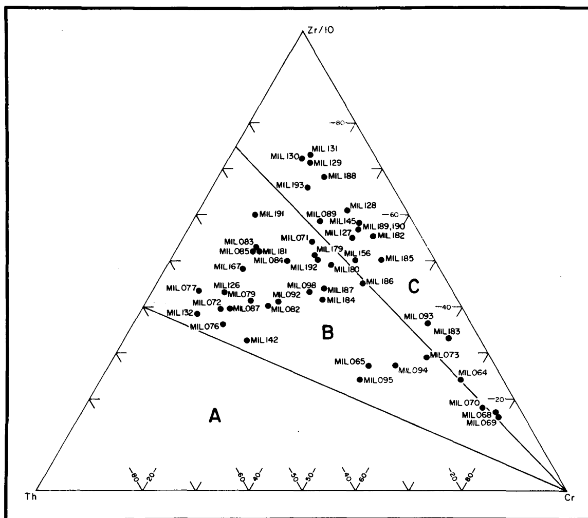
Figure 4. A ternary Zr-Th-Cr discrimination diagram for tuffs from Dillon Quadrangle. Areas A, B, and C drawn from discrimination diagram for flow rocks.
