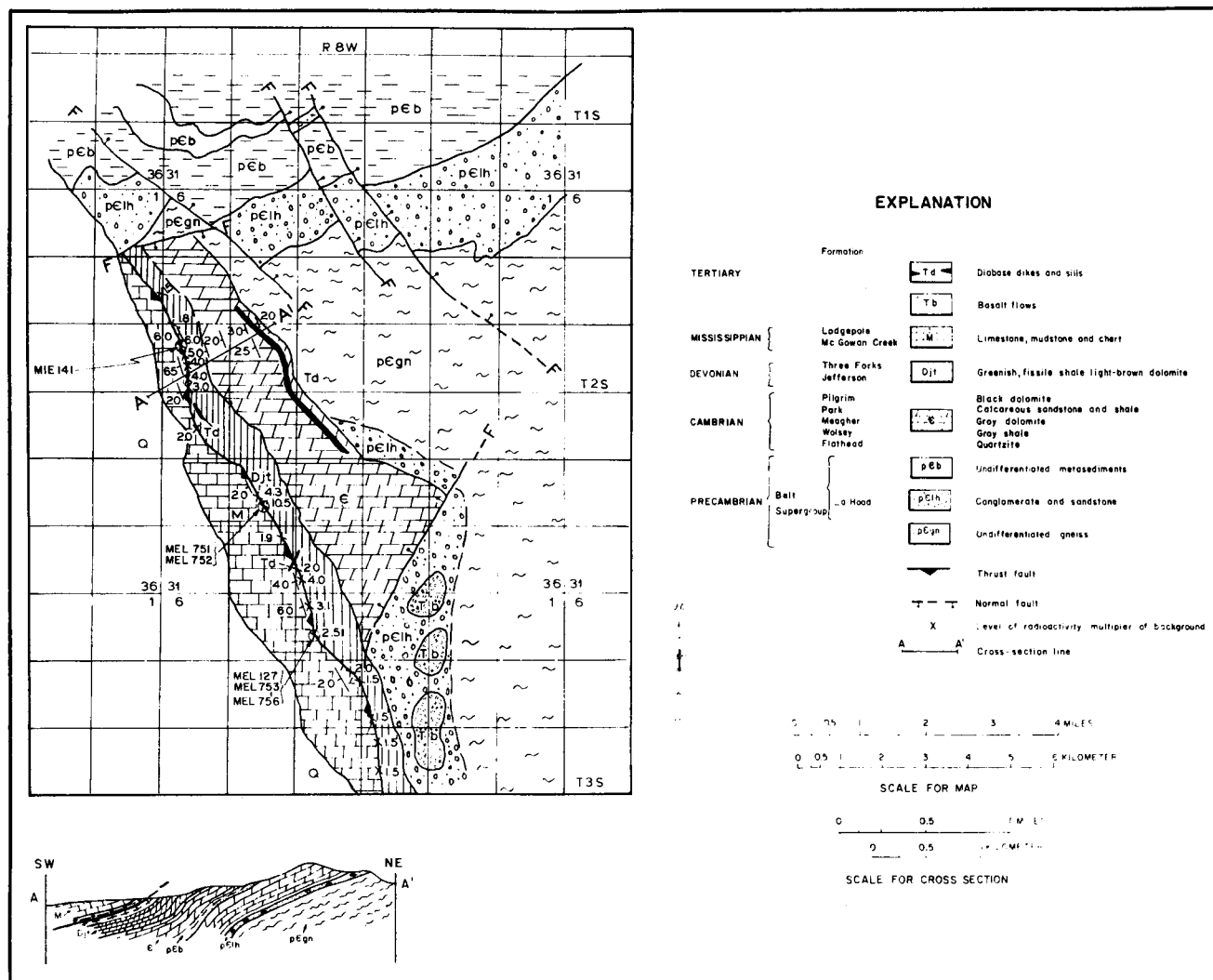
Figure 11. Geologic map and cross section of the Melrose district and adjoining areas.
