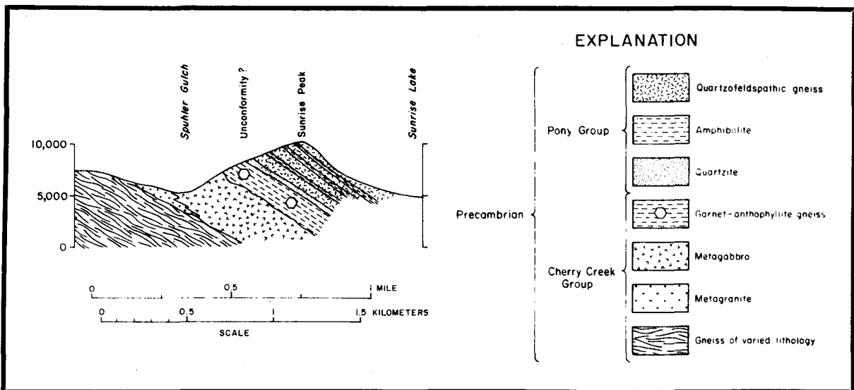
Figure 14. A schematic north-south geologic cross section through Sunrise Peak, Tobacco Root Mountains.
