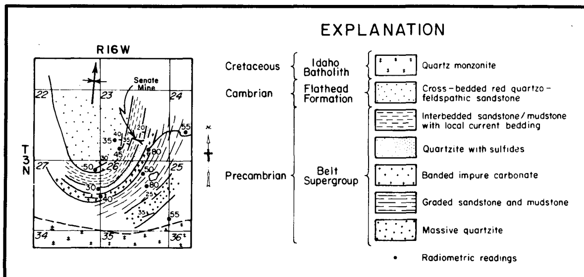
Figure 7. Geologic map of Senate Mine area.
