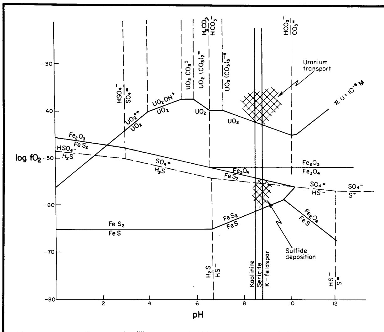
Figure 9. Log fO_2 -pH diagram showing stability fields of iron, sulfide, carbonate, silicate, and uranium species. Activity of total uranium in solution \sim 10^{-6} M. Assumed conditions are: T = 100^\circ\text{C} ; \Sigma\text{CO}_2 = 10^{-2.55} M; \Sigma\text{S} = 10^{-3.1} M; \Sigma\text{K}^+ = 10^{-4.0} M. Thermodynamic data used after Helgeson (1969) and Langmuir (1978). Diagram modified after S. Dodd (pers. comm.).
