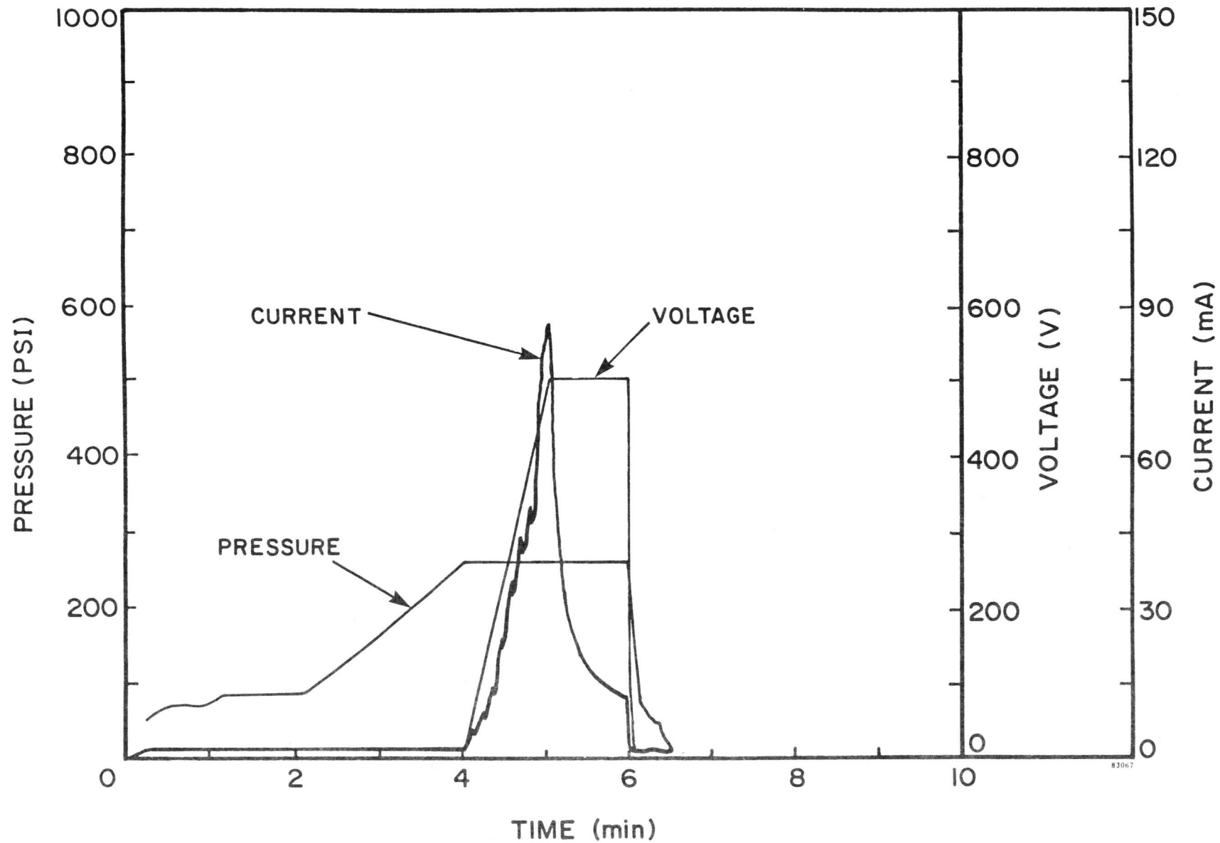
FIGURE 8. OPTIMIZED ESB CYCLE. T=350^{\circ}\text{C} .
