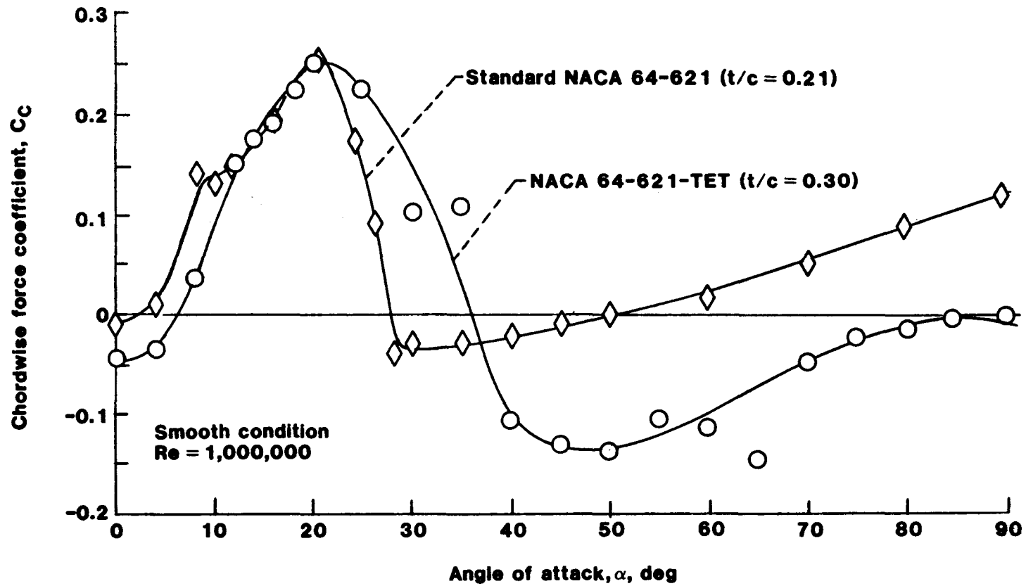
Figure 19.- Chordwise force coefficient comparison, between standard and truncated (TET) NACA 64-621 airfoils.
