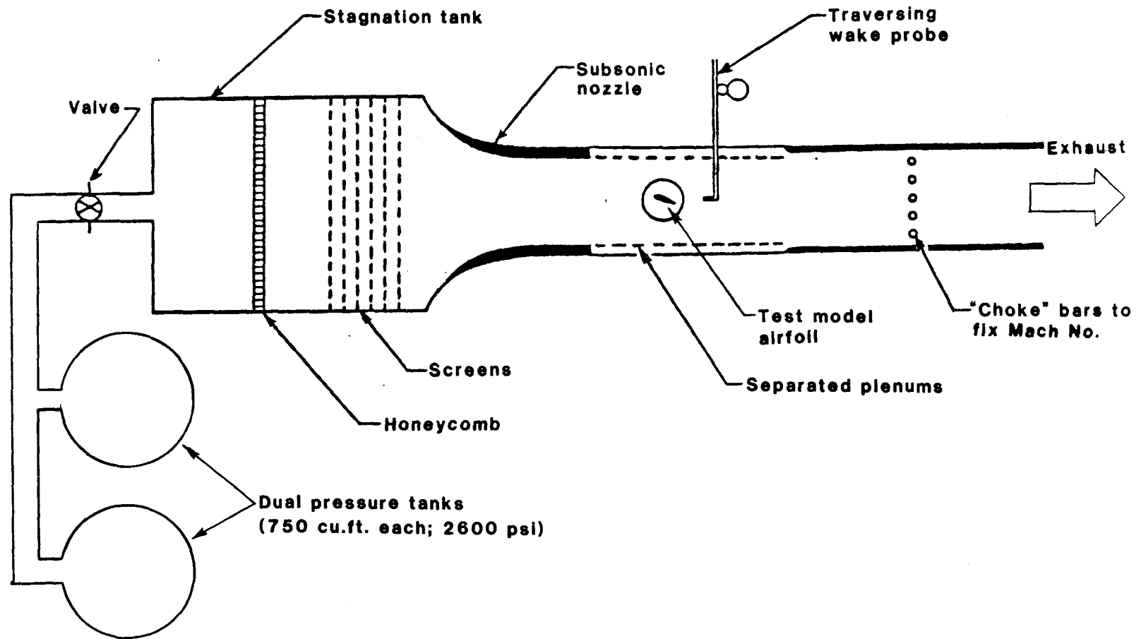
Figure 2.- Schematic view of OSU AARL 6 in. x 22 in. pressurized blow-down wind tunnel.
