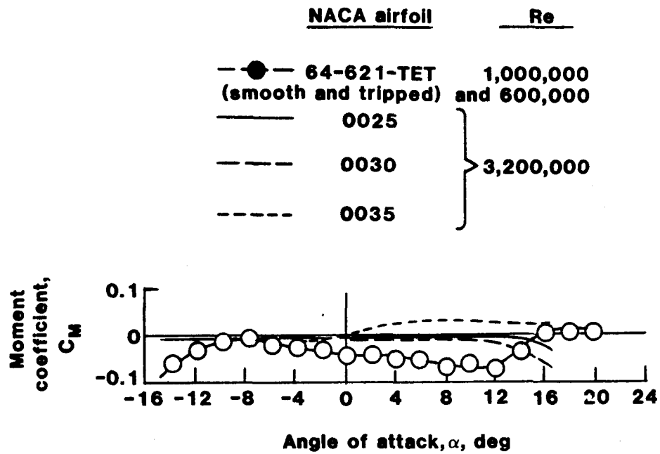
Figure 17.- Moment coefficient comparison, between typical NACA 64-621-TET airfoils and thick NACA 4-Series airfoils (data for NACA 4-Series from Refs. 2 and 3).
