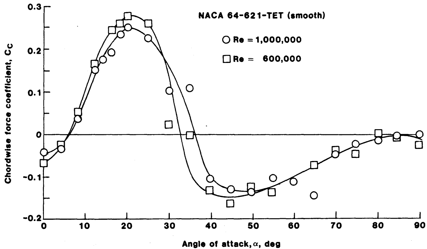
Figure 12.- Chordwise force coefficients for smooth NACA 64-621-TET airfoils at angles of attack up to 90 degrees.
