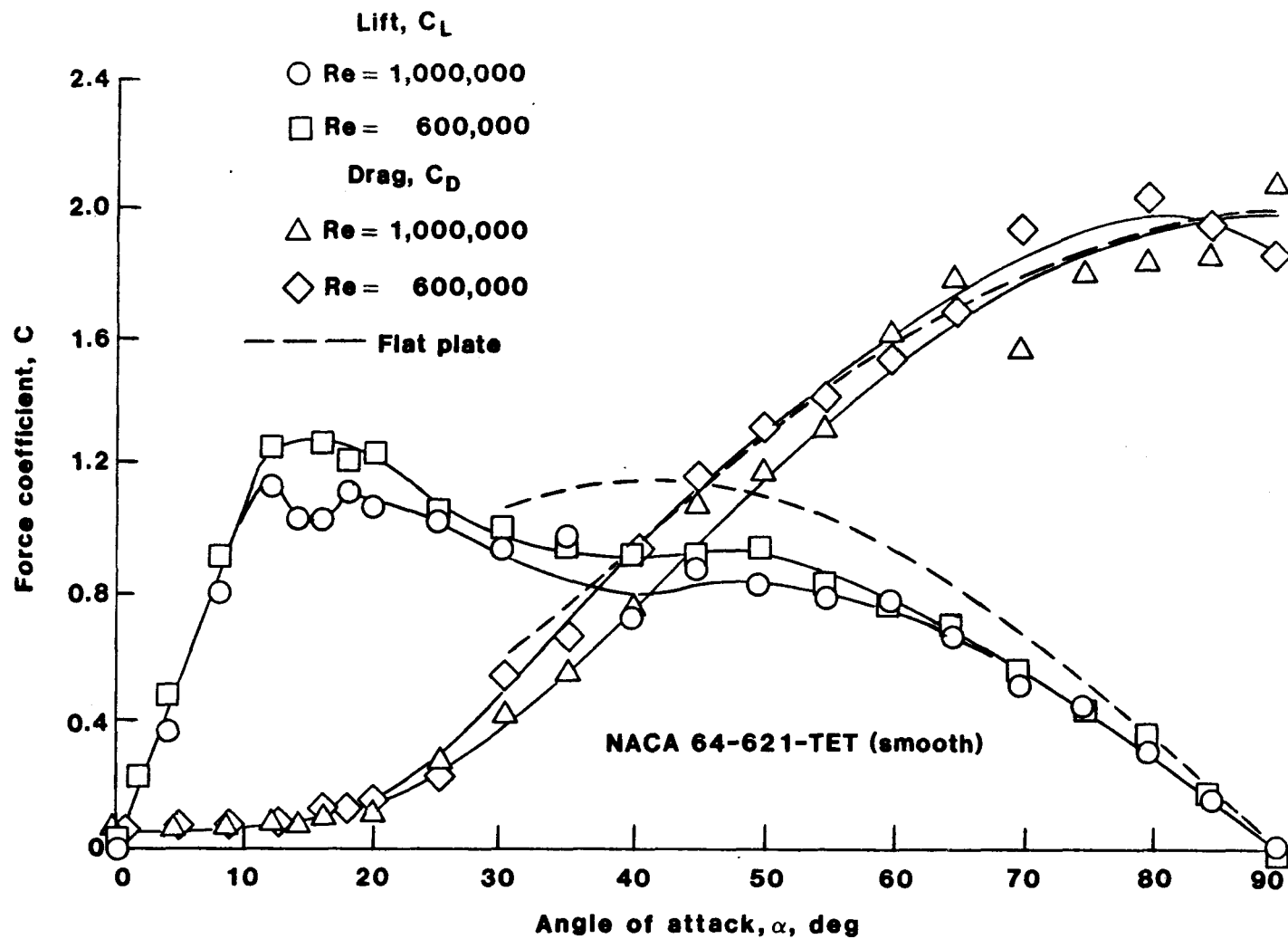
Figure 9.- Lift and drag coefficients for the smooth NACA 64-621-TET airfoil at angles of attack up to 90 degrees.
