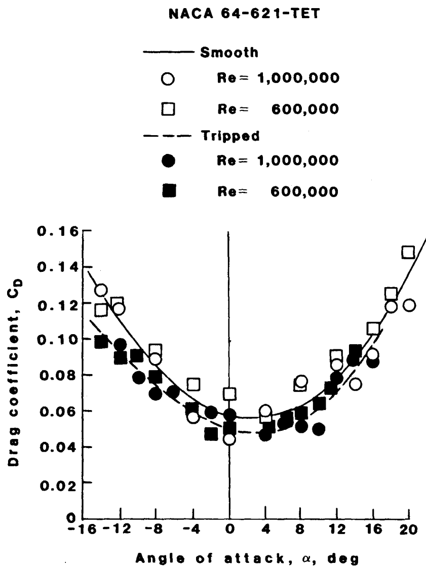
Figure 7.- Drag coefficients for the NACA 64-621-TET airfoils in the smooth and tripped conditions.
