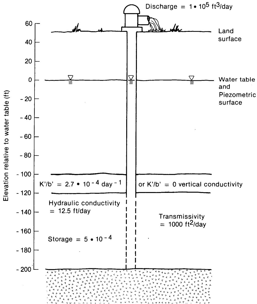
Figure 2. Schematic of aquifer system used to validate the computer code.
