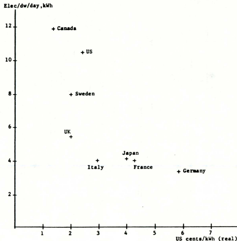
Figure 3. Electricity price and appliance electricity use, 1978
