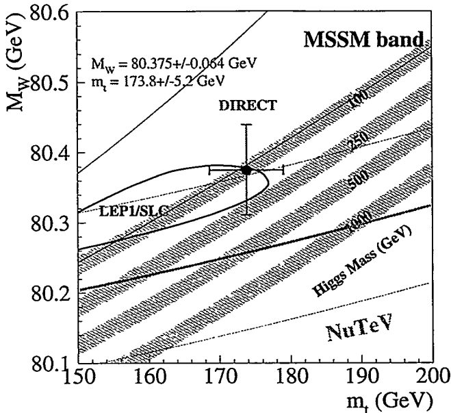
FIG. 15. M_W vs M_{top} . The point is the combined result from direct measurements. Also shown are the allowed regions from LEP1/SLC and NuTeV, the prediction of the minimal supersymmetric model (MSSM), and the Standard Model predictions for Higgs masses from 100 – 1000 \text{GeV}/c^2 .
