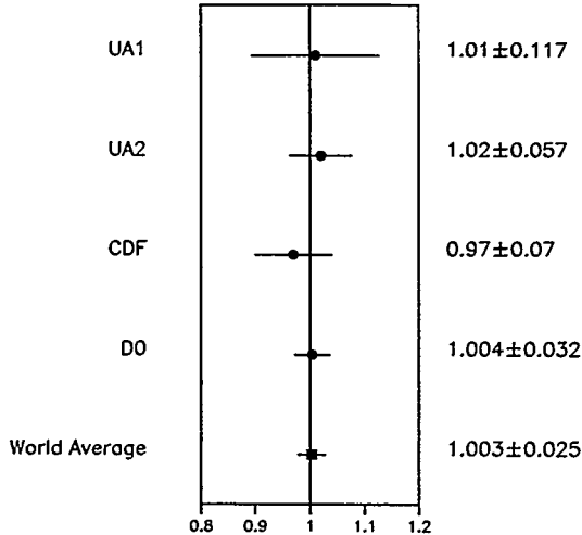
FIG. 2. g_\tau^W/g_e^W from various experiments.
