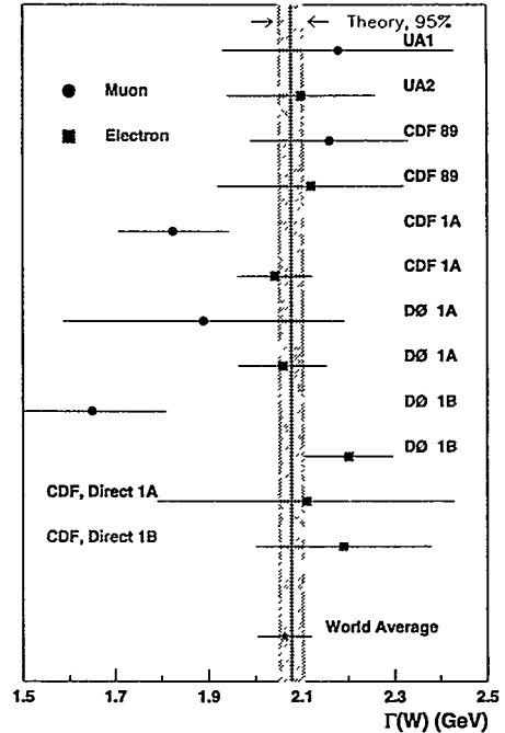
FIG. 3. Summary of W width measurements and comparison with the Standard Model prediction.
