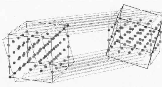
Figure 2: Permutation communication.
