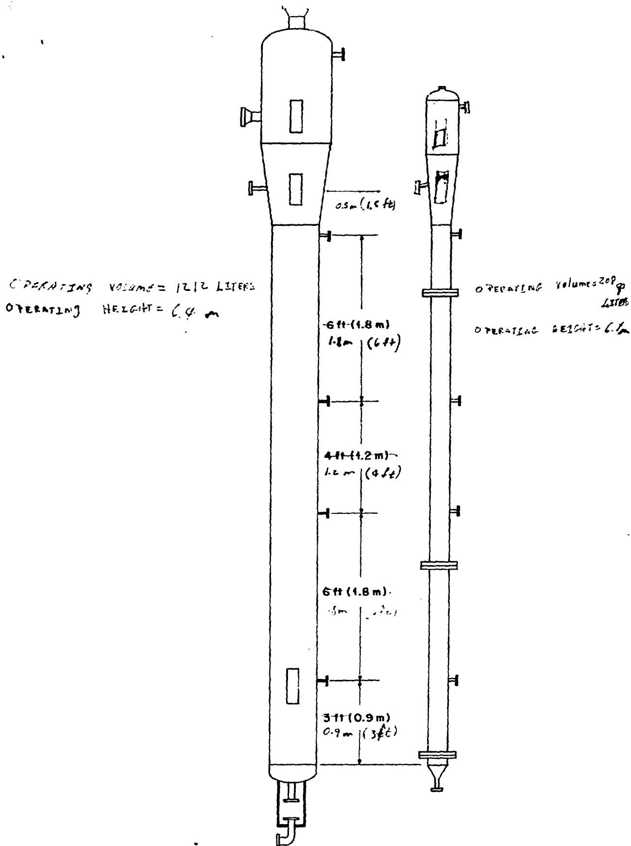
Fig. 3. Comparison of the 20-cm-diam and the 50-cm-diam bioreactors
