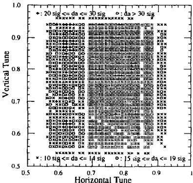
Figure 2. Swamp plot for the HER lattice with beta-bump correction, \beta_y^* = 1.5\text{cm}
