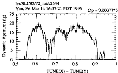
Figure 4. Dynamic apertures along the diagonal line of the tune plane with a fine mesh for a 72° interlaced-sextupole LER lattice
