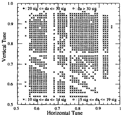
Figure 1. Swamp plot for the HER lattice with interlaced sextupoles, \beta_y^* = 2\text{cm}
