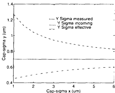
Fig. 5: \Sigma_y , (measured) and \Sigma_y , (effective) versus \Sigma_x .
