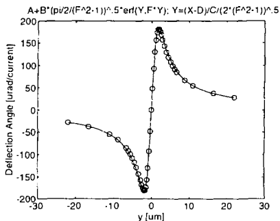
Fig. 3: Simulated Disrupted b-b scan, and deflection fit
