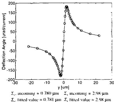
Fig. 6: Simulated Disrupted b-b scan, and Disrupted deflection fit
