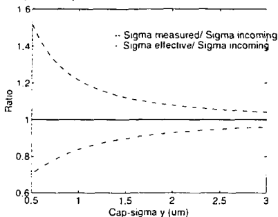
Fig. 4: \Sigma_x , (measured) / \Sigma_x , (incoming) and \Sigma_x , (effective) / \Sigma_x , (incoming) versus \Sigma_x .
