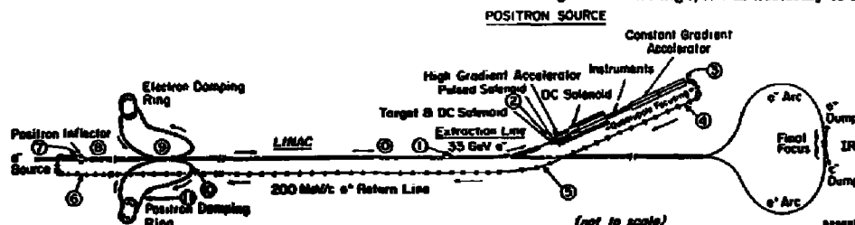
Fig. 11. Schematic diagram of the positron source.
