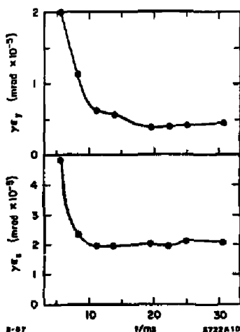
Fig. 5. The emittance of the beam extracted from the electron storage ring as a function of storage time. The vertical emittance \gamma_y is smaller than the horizontal emittance because the ring is operated without coupling.
