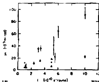
Fig. 3. Electron transverse emittance measurements at 1.21 GeV.
