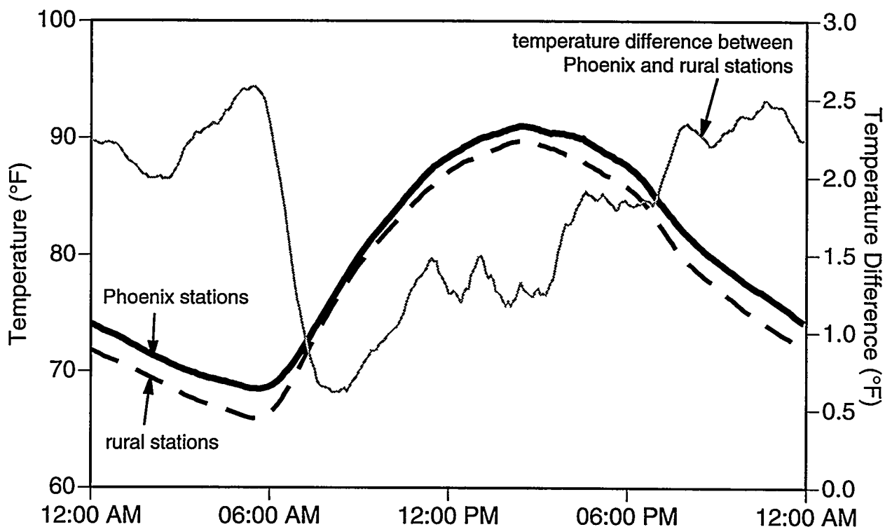
Figure 3: Urban versus rural temperatures at PRISMS sites. The thick solid line is the hourly running average temperature of six weather stations located near the urban center of Phoenix, Arizona. The dashed line is the hourly running average of three rural weather stations. The light solid line represents the difference in temperatures between the two averages.
