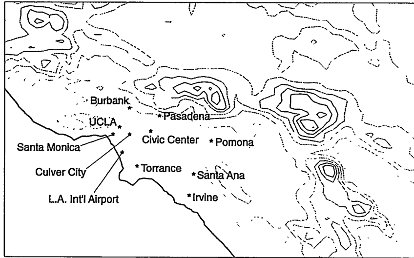
Figure 1: Elevation contour map of Los Angeles area with locations of the cooperative network stations examined. Contours represent changes in elevation of 350 meters.
