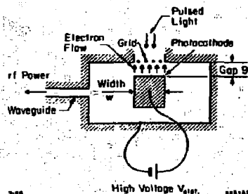
Fig. 2. Micro-lasertron concept as discussed here.
