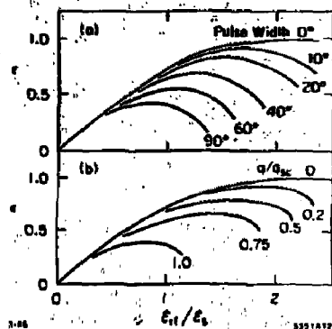
Fig. 11. Efficiency vs. E_{RF}/E_{stat} for a) different pulse lengths and b) different ratios F_{sc} of charge q to the space charge limit q_{sc} .
