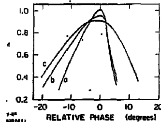
Fig. 10. Efficiency vs. relative phase for a) the magic condition with \mathcal{E}_{RF}/\mathcal{E}_{stat} = 2.0 ; b) \mathcal{E}_{RF}/\mathcal{E}_{stat} = 1.5 ; c) \mathcal{E}_{RF}/\mathcal{E}_{stat} = 1.0 .
