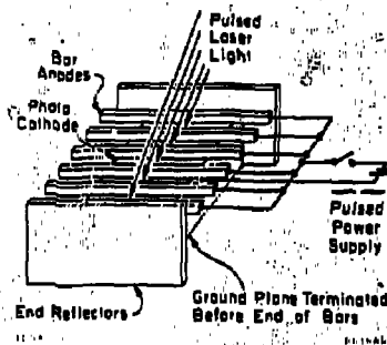
Fig. 5. Micro-lasertron geometry, including cavity end design.
