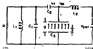
Fig. 6. Equivalent circuit of micro-lasertron.
