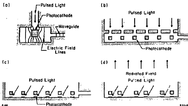
Fig. 4. Realizations of the micro-lasertron: a) single cavity, b) multi cavity, c) grating cavity, d) modification to grating cavity to couple to outgoing wave.
