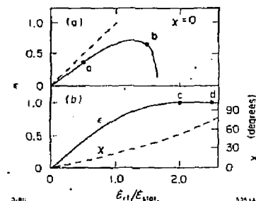
Fig. 7. Efficiency vs. strength of RF field a) for phase advance \chi = 0 and b) phase advance adjusted to give maximum efficiency.
