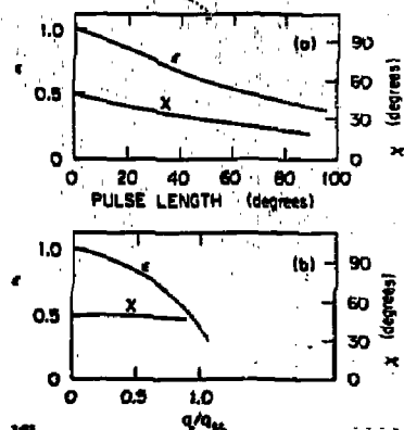
Fig. 12. Maximum efficiencies and corresponding phase advances \chi as a function of a) pulse length and b) charge.
