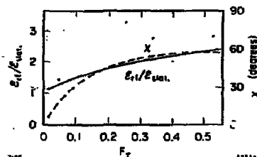
Fig. 9. Values of \mathcal{E}_{RF}/\mathcal{E}_{stat} and the phase advance \chi to give the 'magic' condition for different transit time factors F_T .
