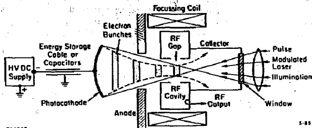
Fig. 3. The conventional lasertron concept.
