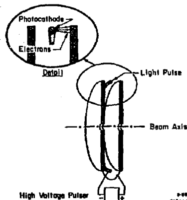
Fig. 1. Switched power accelerator concept as proposed by W. Willis (Ref. 1).
