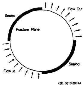
Figure 1. Flow path in quadrant flow technique.
