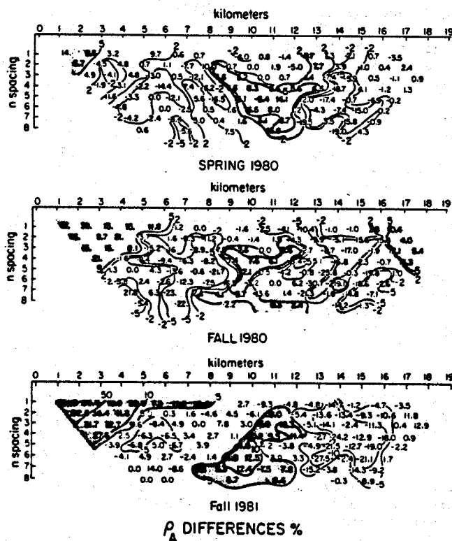
Figure 1. Resistivity pseudosections measured over the Cerro Prieto Geothermal Field shown as percent changes from the 1979 baseline data set.
