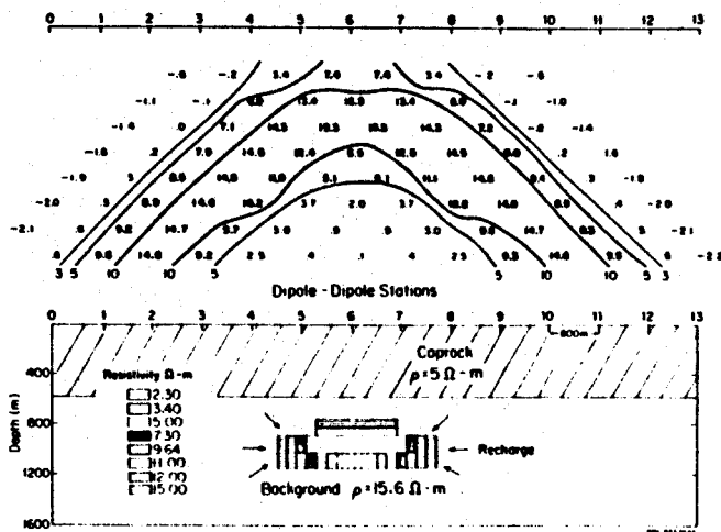
Figure 7. Resistivity pseudosections for reservoir with vertical and lateral recharge (percent changes).
