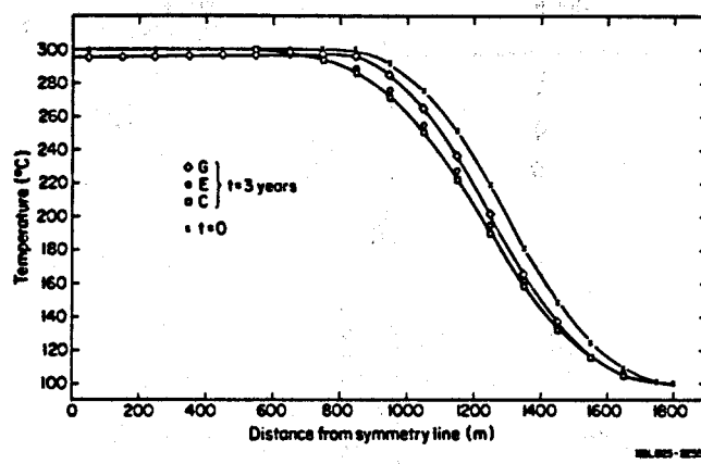
Figure 3. Temperature profiles for two-dimensional model.
