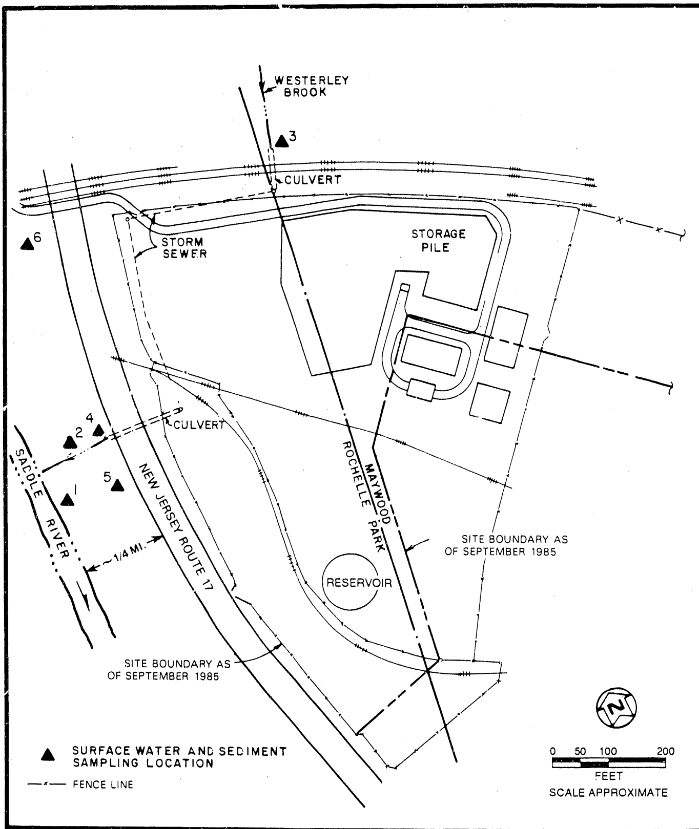
FIGURE 3-2 SURFACE WATER AND SEDIMENT SAMPLING LOCATIONS IN THE VICINITY OF MISS
