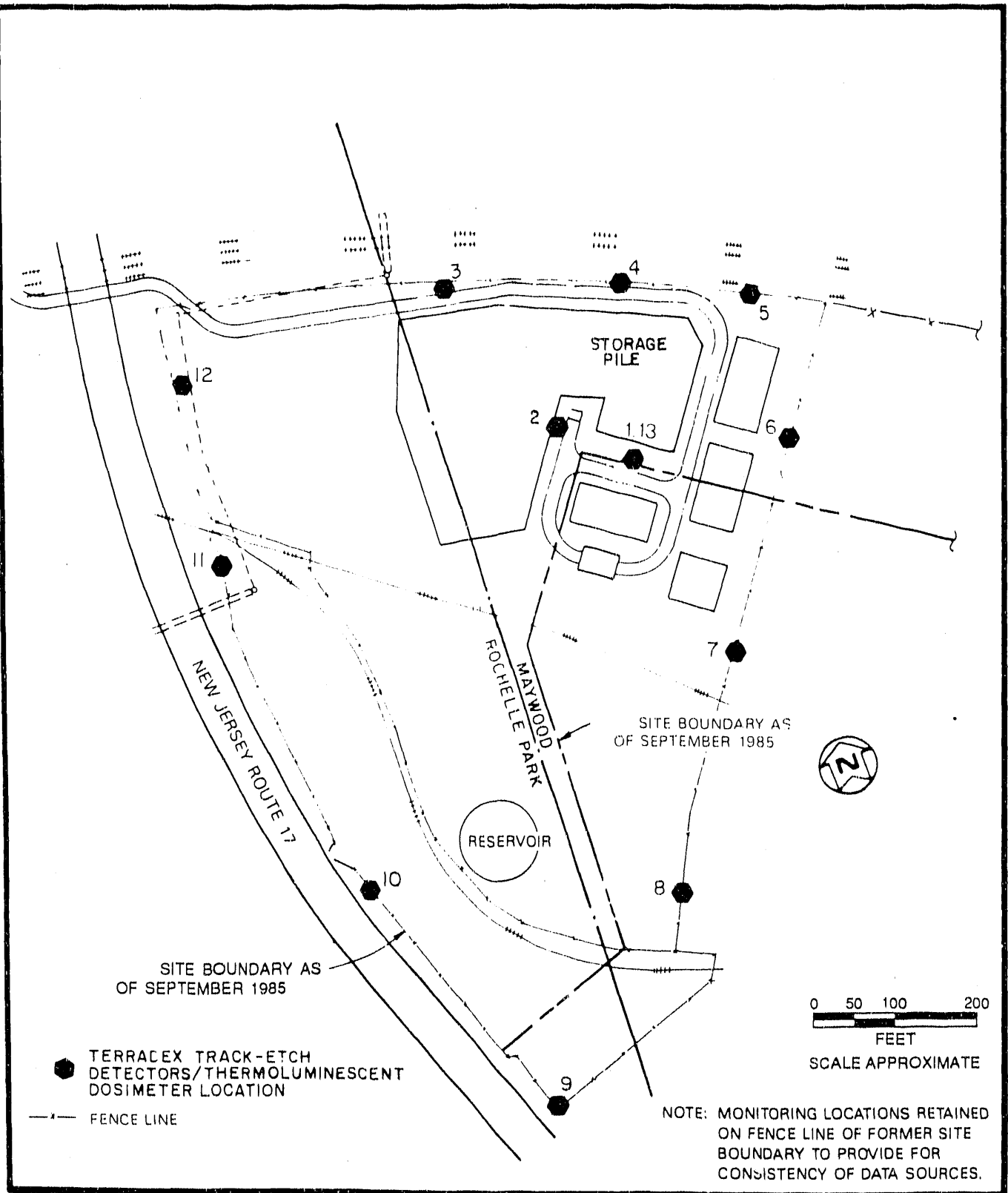
FIGURE 3-1 RADON AND EXTERNAL GAMMA RADIATION MONITORING LOCATIONS AT MISS
