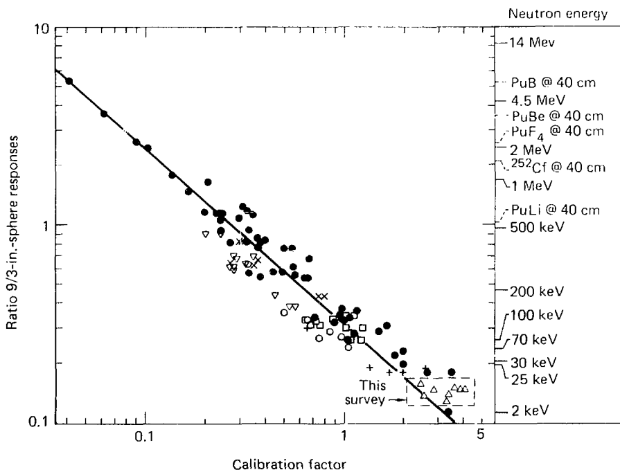
Fig. 2. Curve Used to Obtain the Calibration Factor for Albedo Neutron Dosimeters
