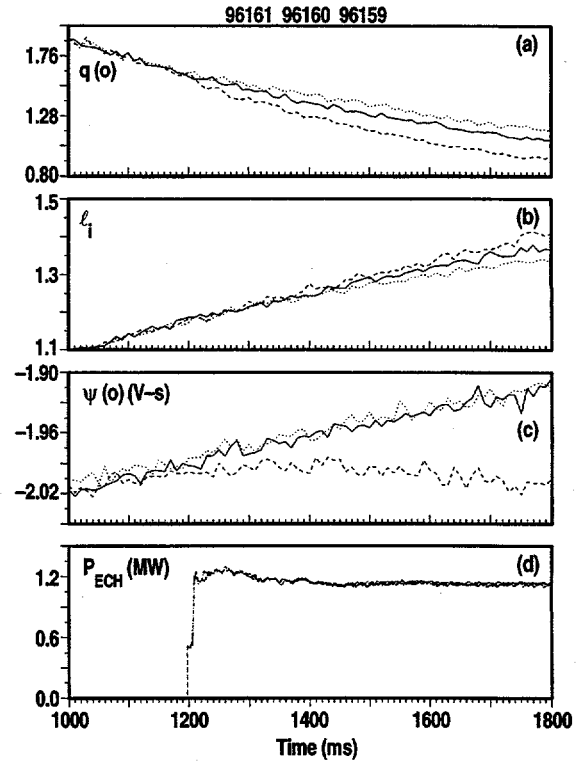
Fig. 3. The central safety factor q(0) , the internal inductance l_i , the poloidal flux at the plasma center, and the applied ECH power, for three discharges. In #96161 there is no ECH power, in #96160 (dashed line) there is central co-ECCD (1.03 MW), and in #96159 (dotted line) there is co-ECCD (1.07 MW) applied at a normalized minor radius near 0.4. The toroidal field is 1.97 T, the line-averaged electron density is 1.7 \times 10^{19} \text{ m}^{-3} , and the plasma current is 1.0 MA. In all three cases the neutral beam power is 2.5 MW.
