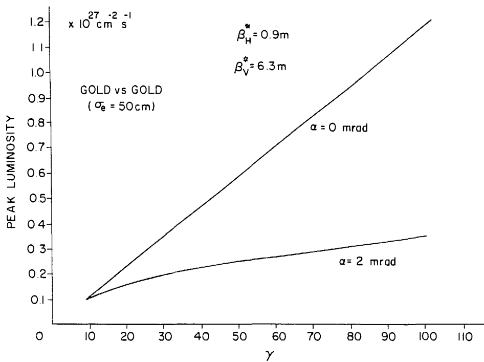
Fig. 27. Peak luminosity vs. energy ( \gamma )
