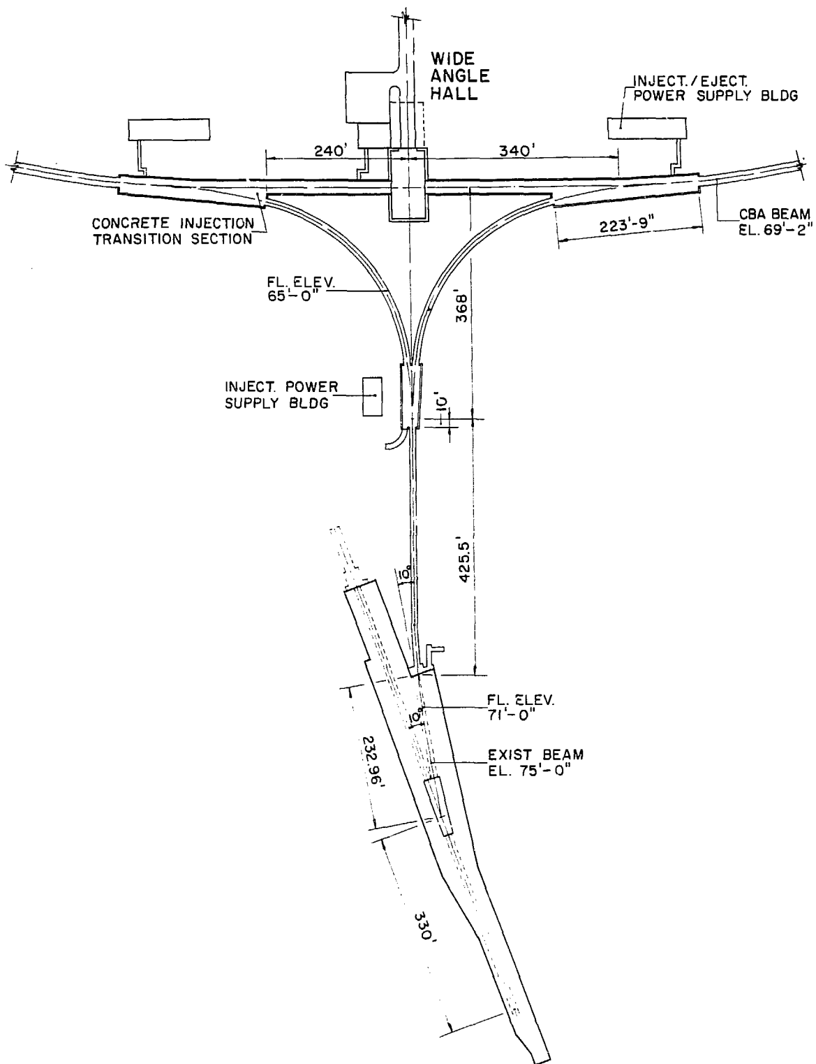
Fig. 8. Accelerator injection plan
