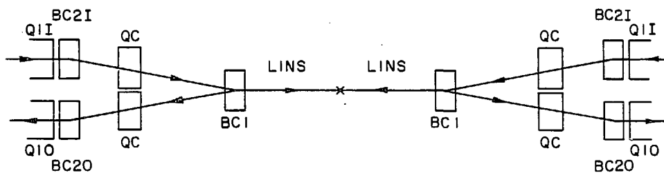
Fig. 14b. Head-on collision, \alpha = 0
