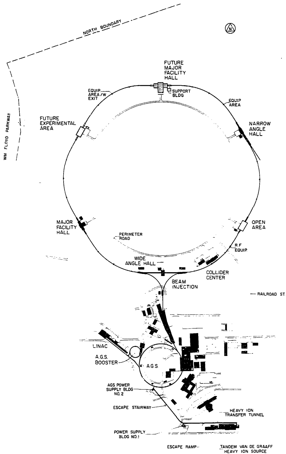
Fig. 1. Layout of RHIC project - collider and source
