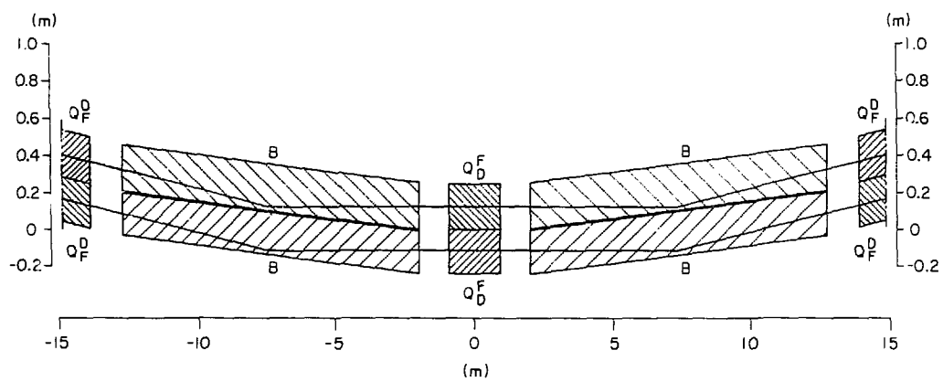
Fig. 10. RHIC regular cell pair
