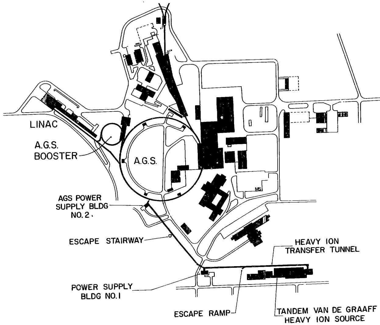
Fig. 2. Injection system for collider
