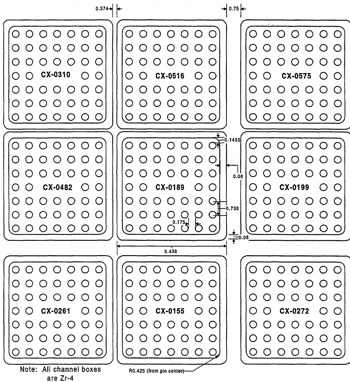
Fig. B.9. Suggested cycle 1 bundle arrangement.
