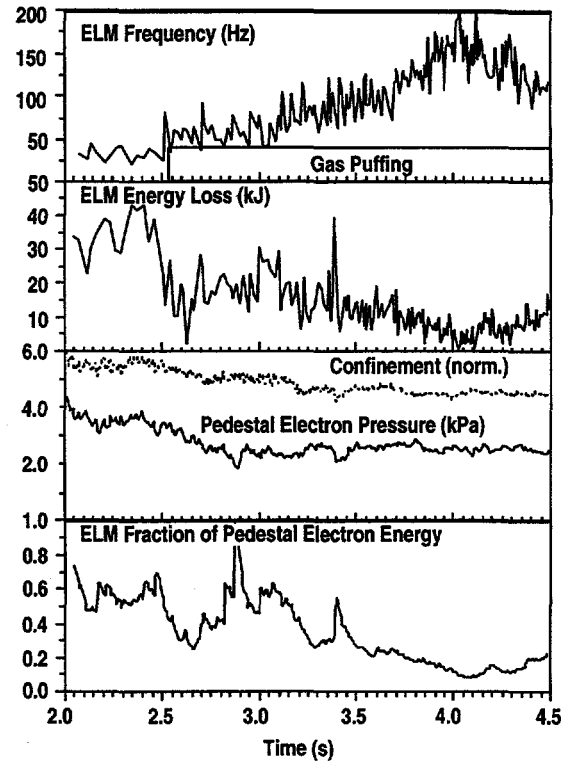
Fig. 3. The ELM and edge pedestal characteristics on DIII-D with gas puffing. Shown are the ELM frequency, the energy loss of individual ELMs, the pedestal electron pressure, the normalized confinement time and the fraction of pedestal energy lost at each ELM.
