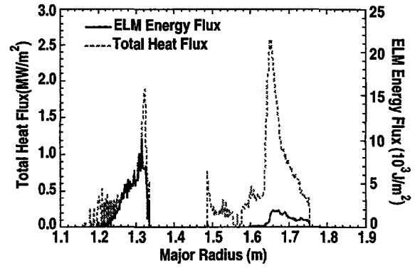
Fig. 2. ELM divertor energy deposition profile for ASDEX-Upgrade.
