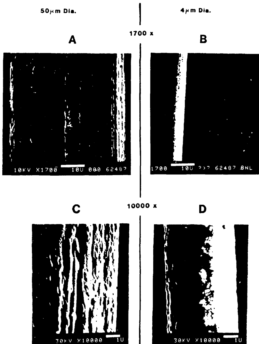
FIGURE 4. SEM pictures of the wire cathodes before installation in the cells. Figs. A and B are the 50 \mu m diameter and 4 \mu m diameter wires, respectively, magnified 1700 times. Figures C and D are the same wires magnified 10000 times. Ridges created by the manufacturing process and shallower gold granularities are evident.
