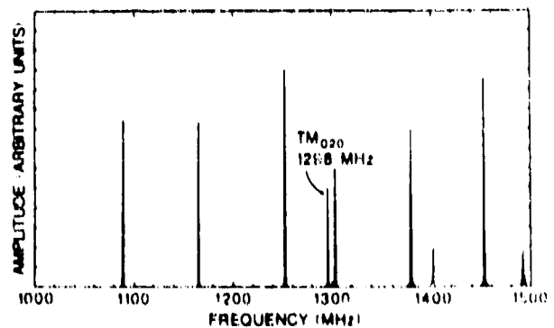
Fig. 3. Measured cavity mode spectra
