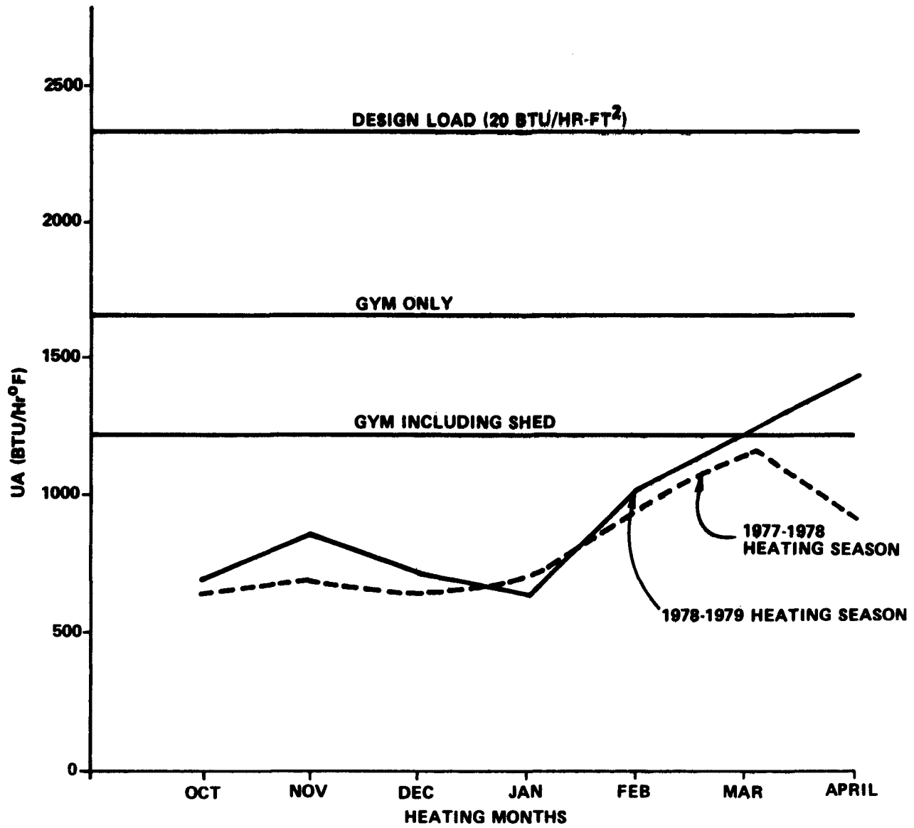
Figure 5.3.4-1. BUILDING HEAT LOSS COEFFICIENT DETERMINATION
