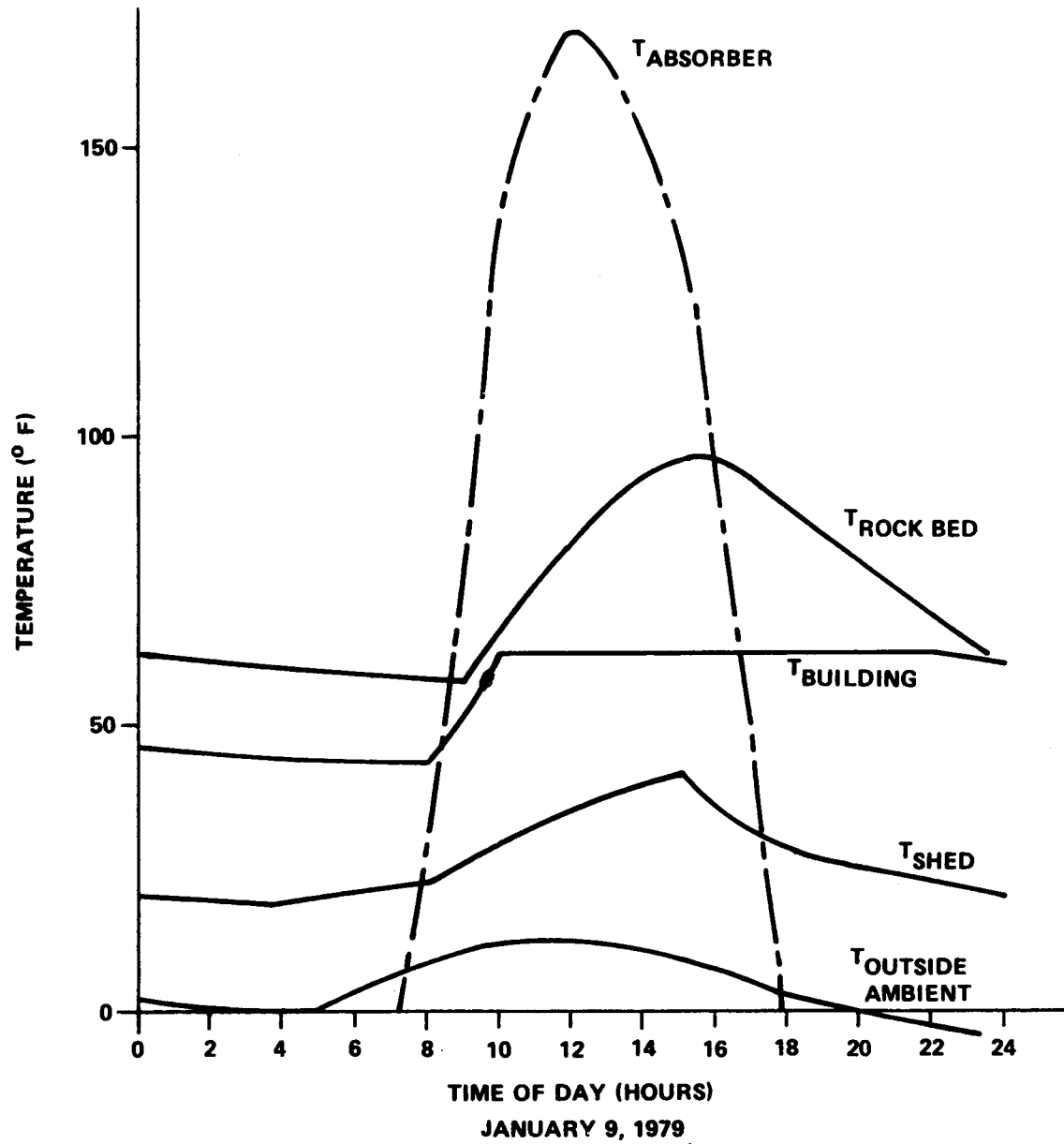
Figure 5.3.2-1 SOLAR SYSTEM AND RECREATIONAL BUILDING TEMPERATURE PROFILES
