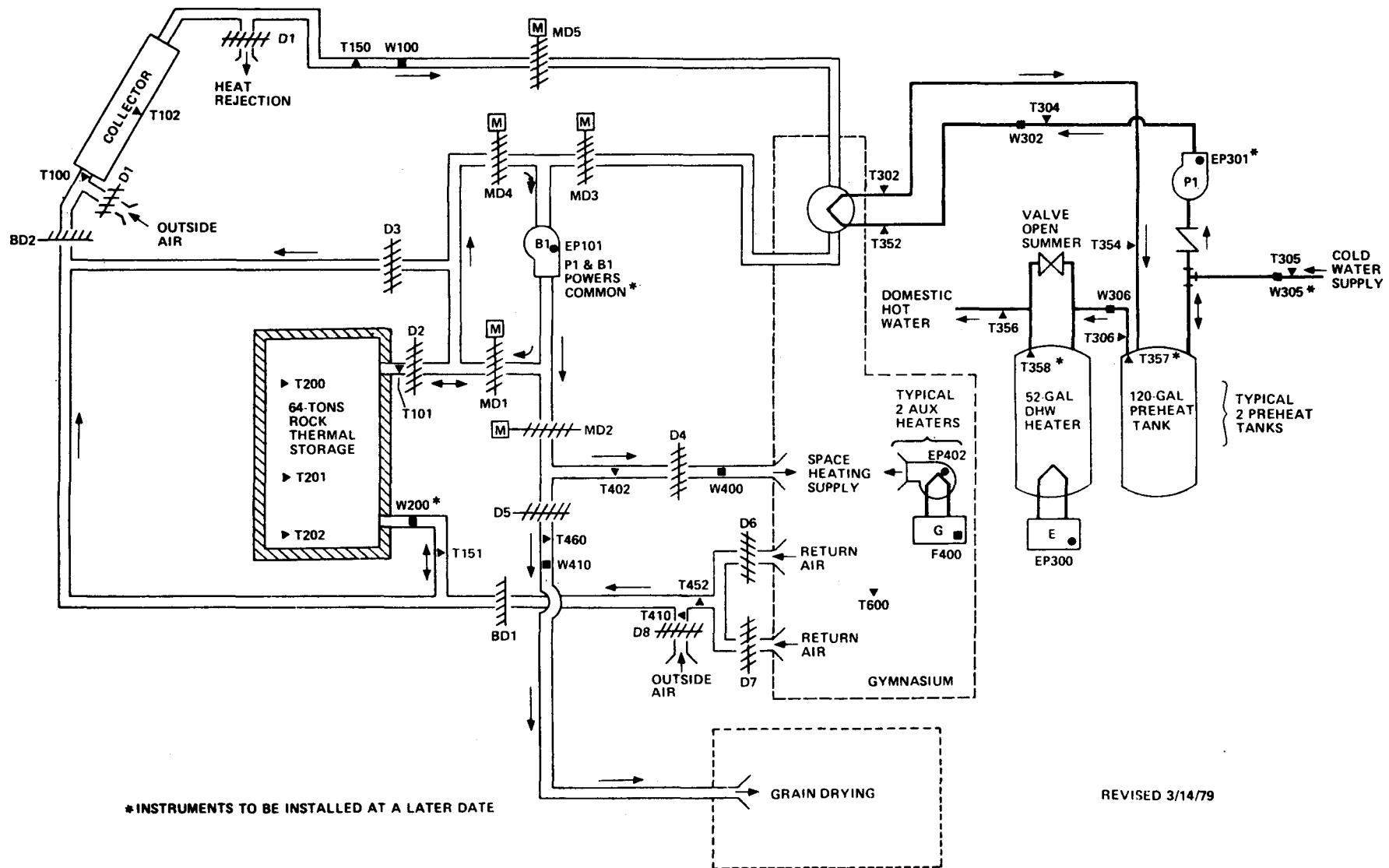
Figure 3-1. SCATTERGOOD SCHOOL SOLAR ENERGY SYSTEM SCHEMATIC
