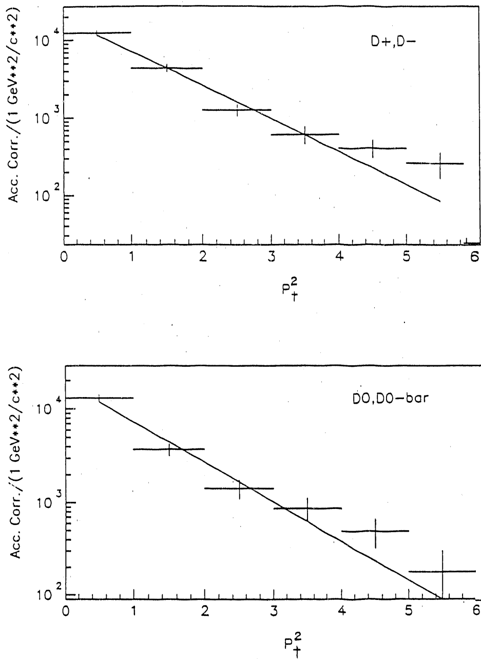
Figure 3: Acceptance corrected p_T^2 distributions, with the fit representing e^{-bp_T^2} for (a) D^+ \rightarrow K^- \pi^+ \pi^+ and (b) D^0 \rightarrow K^- \pi^+ ; b = 0.98 \pm 0.07 and b = 0.95 \pm 0.09 respectively.
