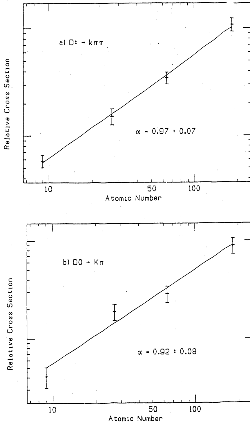
Figure 4: Nuclear A dependence for the (a) D^+ and (b) D^0 signals; the fits represent A^\alpha . The values for \alpha are \alpha = 0.97 \pm 0.07 for the D^+ and \alpha = 0.92 \pm 0.08 for the D^0 .
