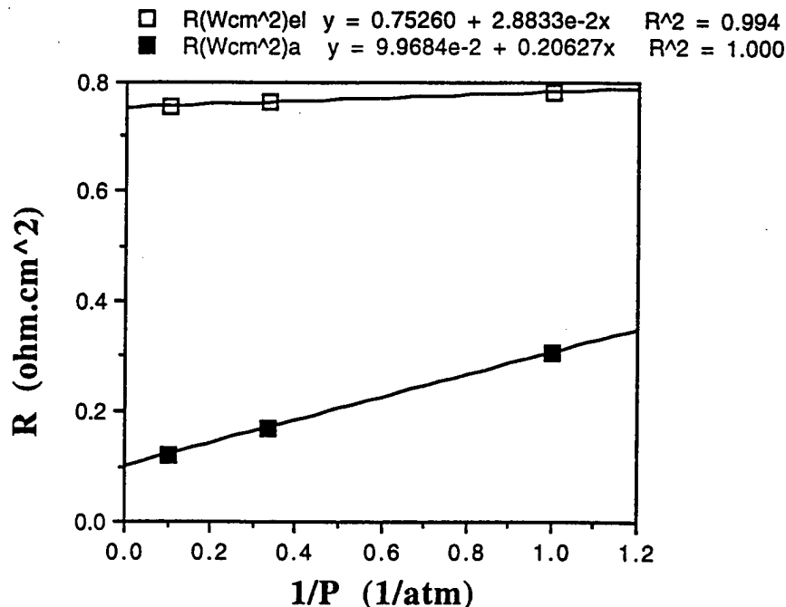
Figure #3: Plot of the calculated cell resistance, inclusive of concentration polarization, vs. 1/\text{pressure} , for cathode-supported and electrolyte-supported cells. The slope of the plot is a measure of the effect of pressure on concentration polarization.
