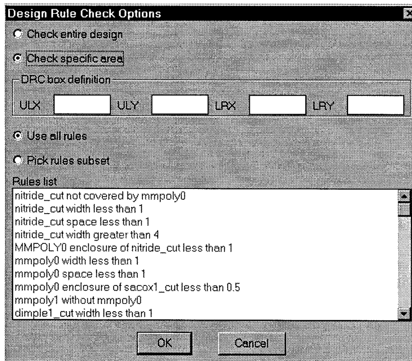
Figure 3. Design Rule Check Options Dialog Box
