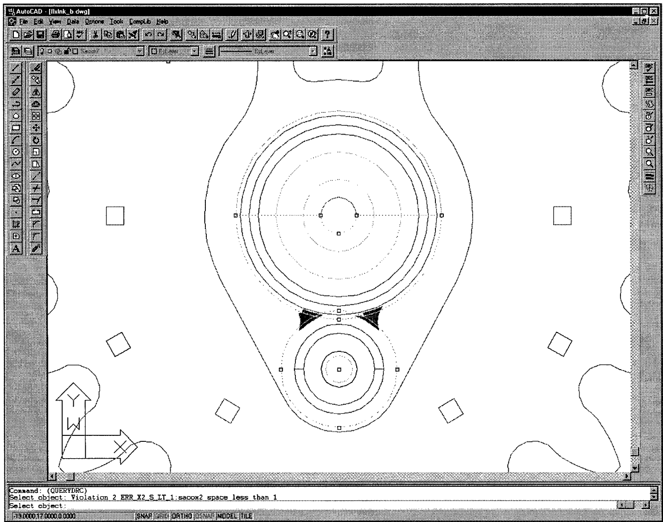
Figure 7. DRC Result Example - Space Violation
