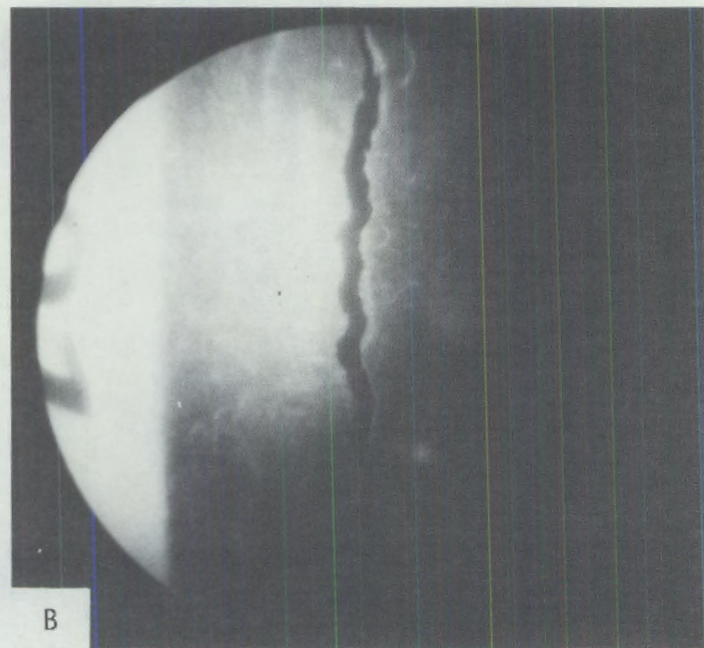
FIGURE 6. Photographs of Sample Steam Generator Tube Taken Through the Lenox Borescope: A) Scope to Subject Distance - 4\text{-}1/8 "; B) Scope to Subject Distance - 9/16 "
