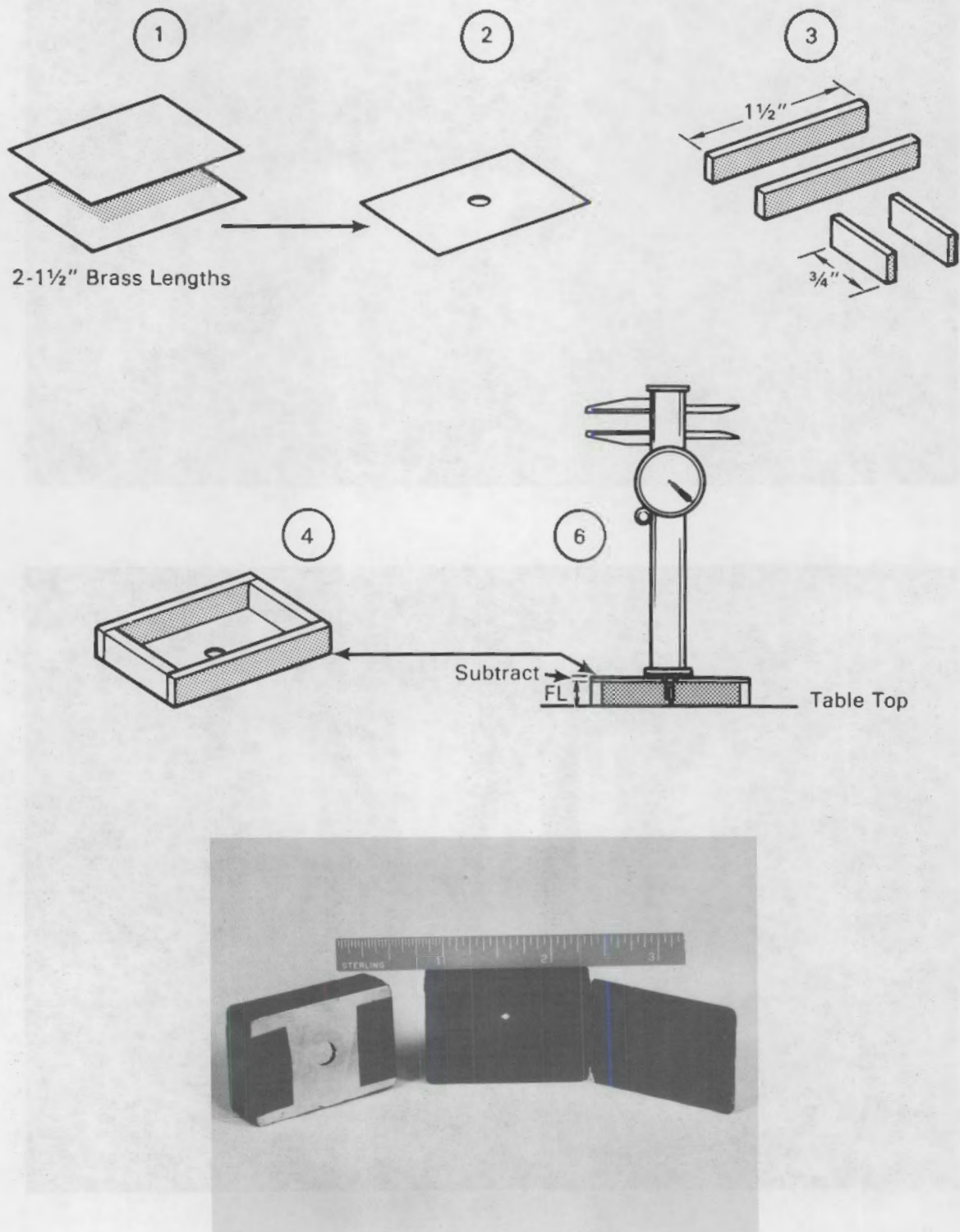
FIGURE 14. Procedure for Fabricating Rectangular Pinhole Camera
