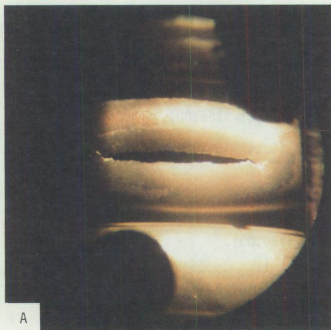
FIGURE 8. Photographs Taken Through the \frac{1}{2} " Diameter Periscope: A) Looking Up at U-Bends (Scope to Subject Distance - 2" - 2- \frac{1}{2} ""); B) Showing Tube Support Plate Intersection and Dent in Steam Generator Tube (Scope to Subject Distance - \frac{3}{4} " - 1")
