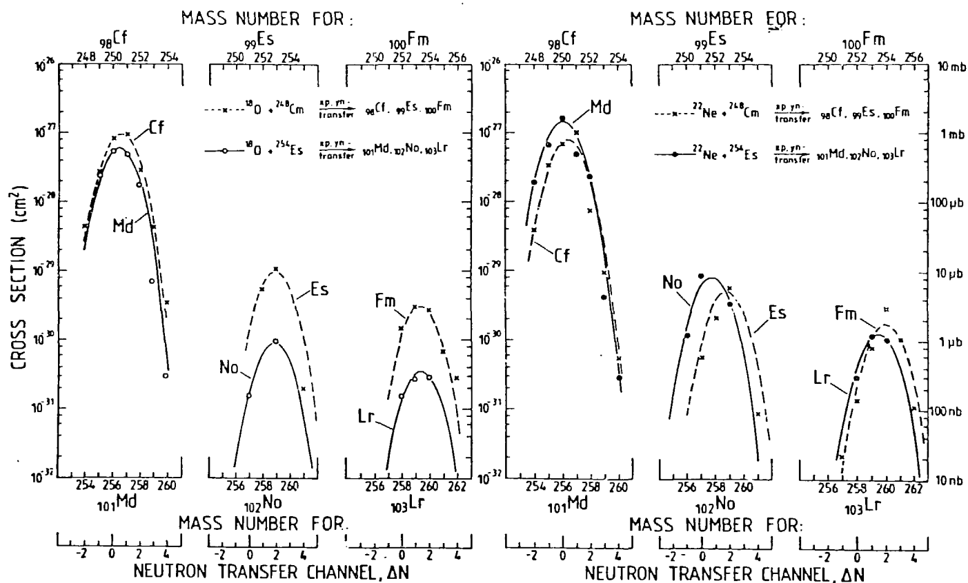
Fig.2. Comparison of measured isotopic cross sections for two-, three- and four-proton and x-neutron ( \Delta N ) transfer products from ^{248}\text{Cm} and ^{254}\text{Es}
