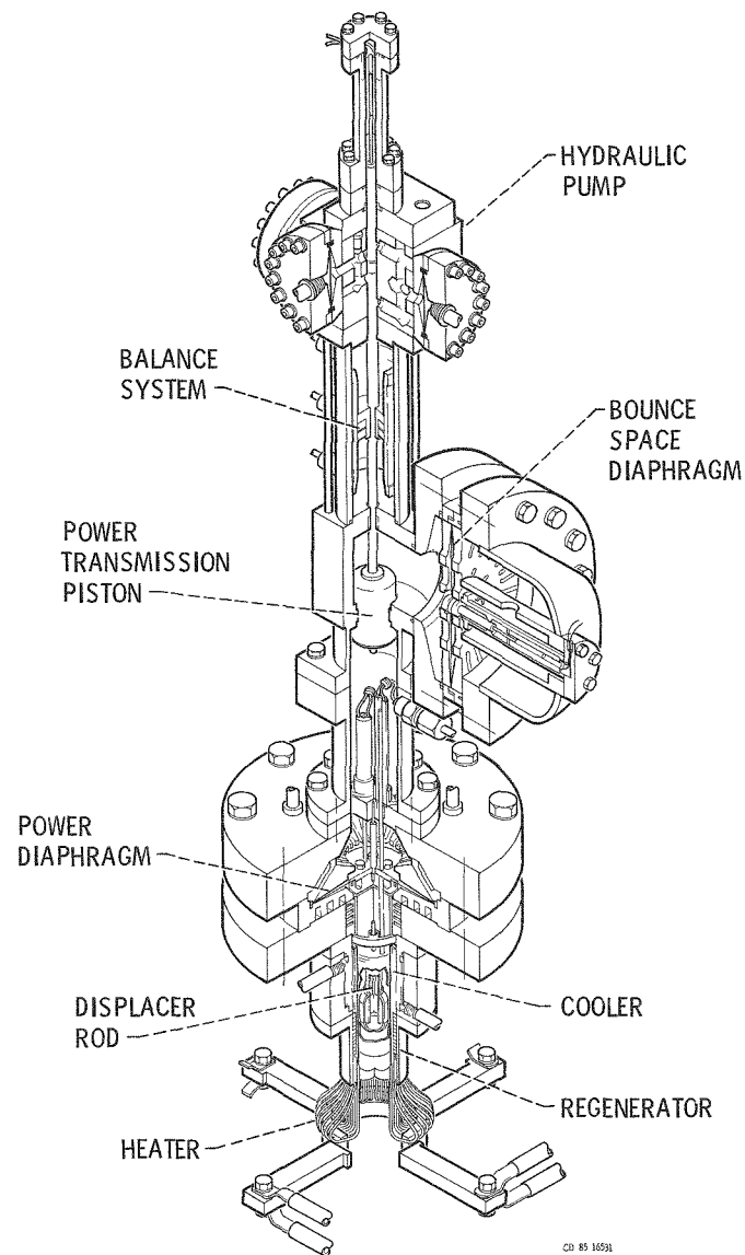
Figure 4. - RE-1000 free-piston Stirling with hydraulic output.
