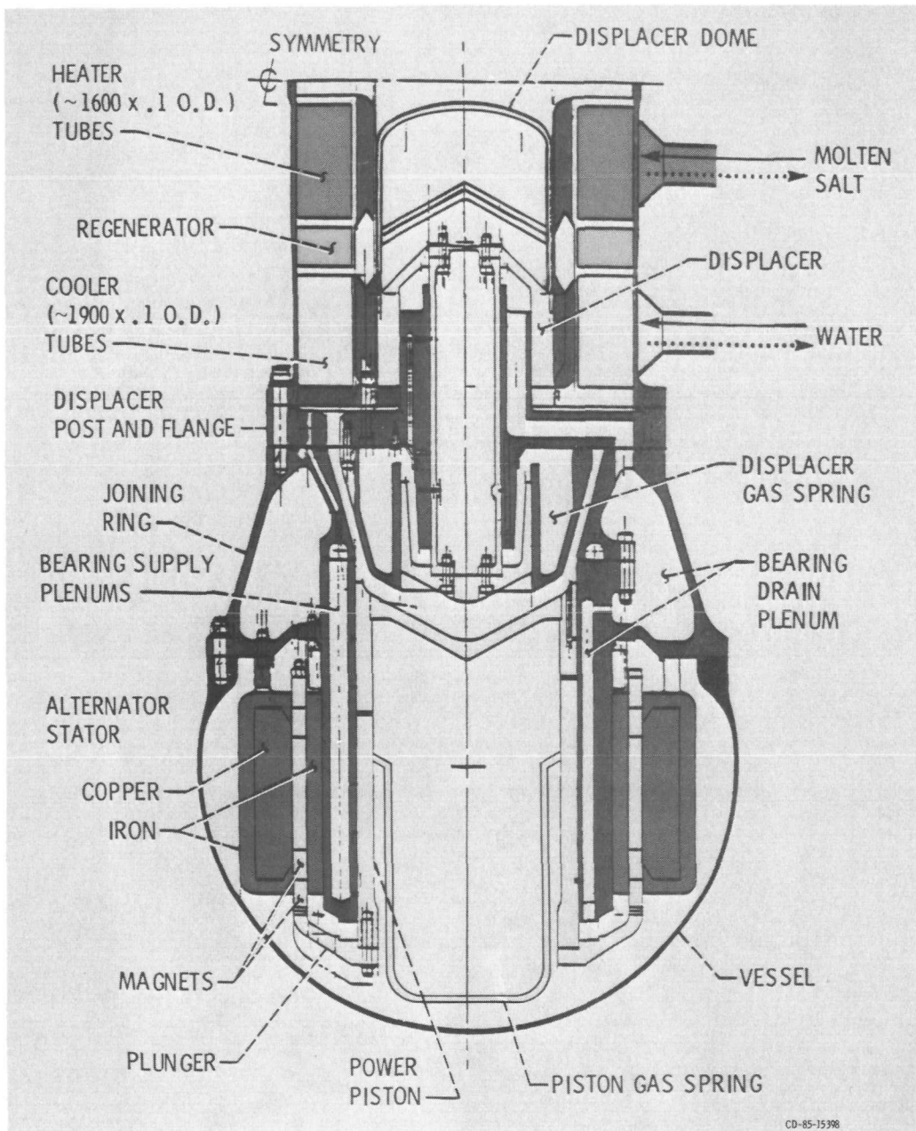
Figure 11, - 25 kWe SPDE.
