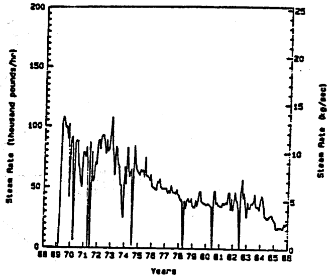
Figure 4. Steam flowrate curve for a well at The Geysers.
