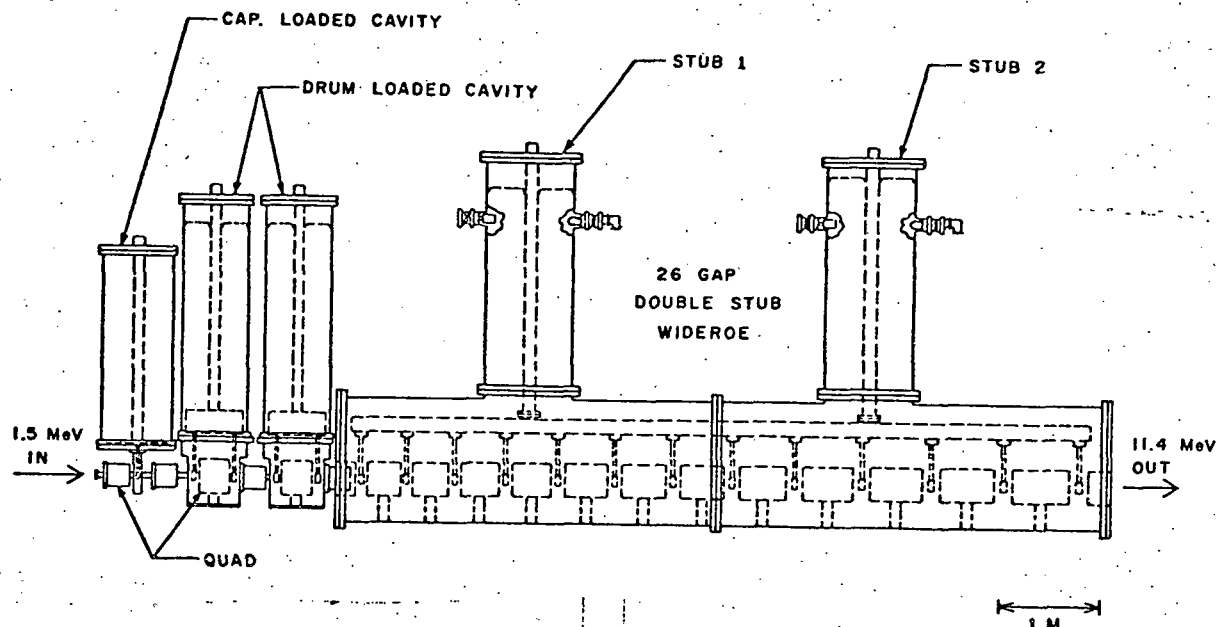
Fig. 1 12.5 MHz Low Beta Linac.
