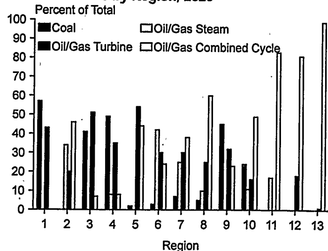
Figure 5. Plant Types Setting Marginal Electricity Prices by Region, 2020
