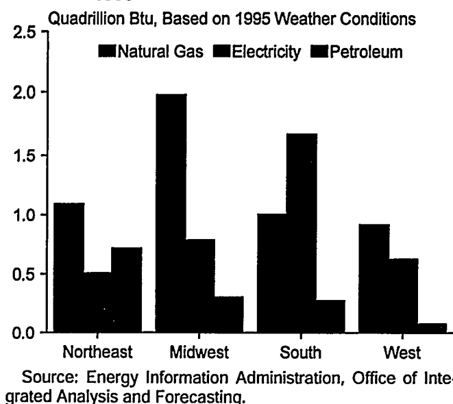
Figure 3. Residential Sector Delivered Energy Consumption by Major Fuel and Region, 1995
