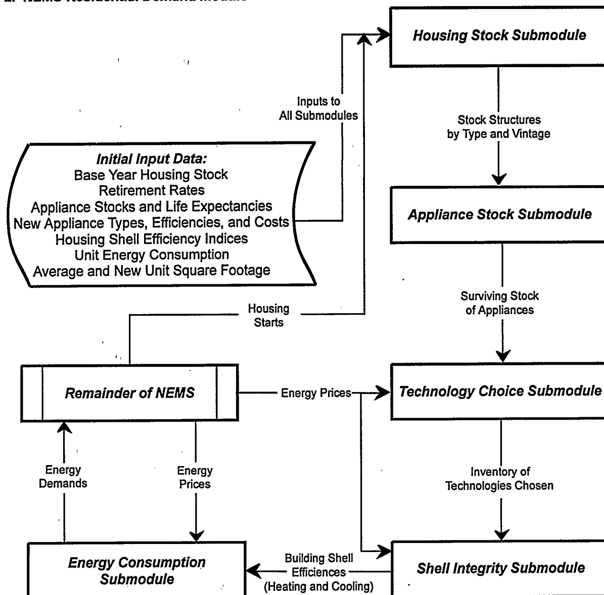
Figure 2. NEMS Residential Demand Module
