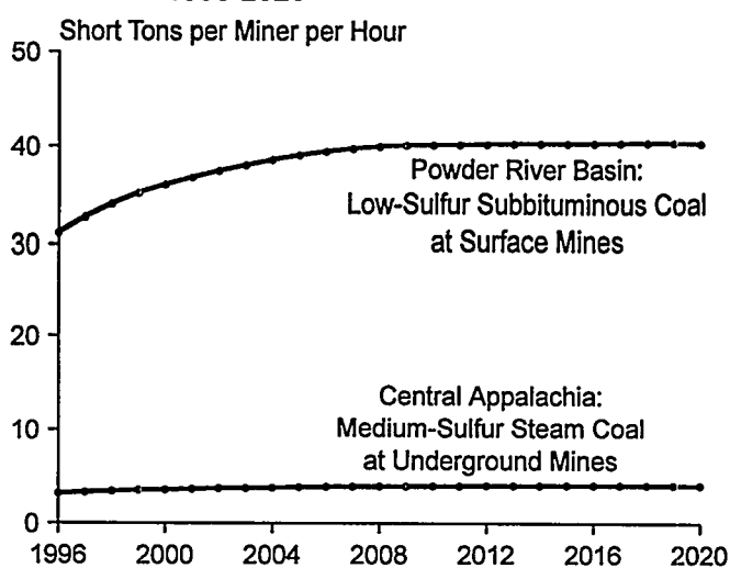
Figure 11. Average Coal Mine Labor Productivity for Selected CMM Supply Curves, 1996-2020
