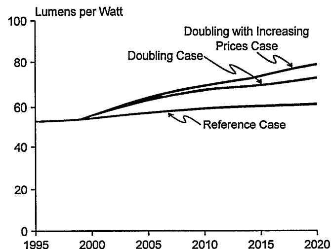
Figure 11. Commercial Sector Lighting Efficiencies, 1995-2020
