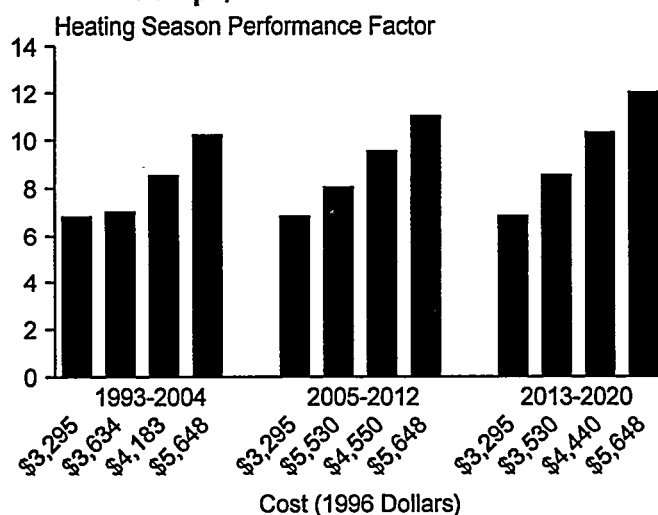
Figure 5. Installed Costs and Efficiencies of Heat Pumps, 1993-2020
