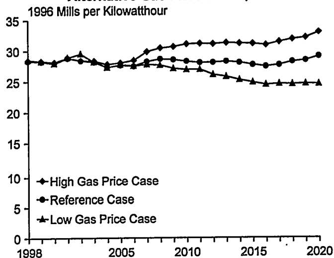
Figure 6. National Average Generation Prices in Alternative Gas Price Cases, 1998-2020
