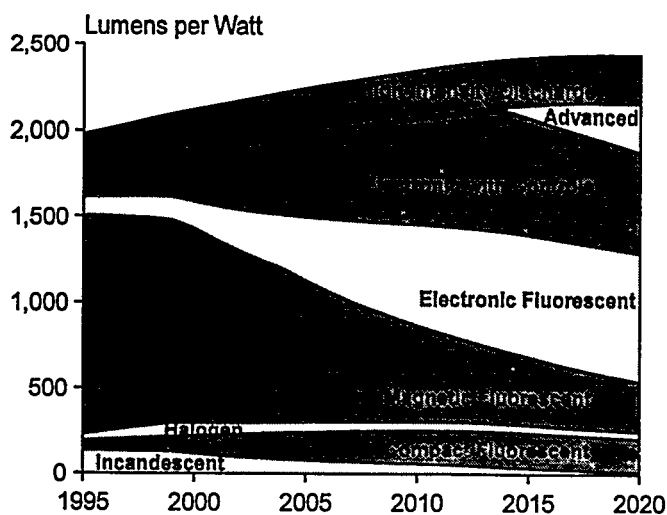
Figure 14. Lighting Service Demand by Technology, Doubling with Increasing Prices Case, 1995-2020
