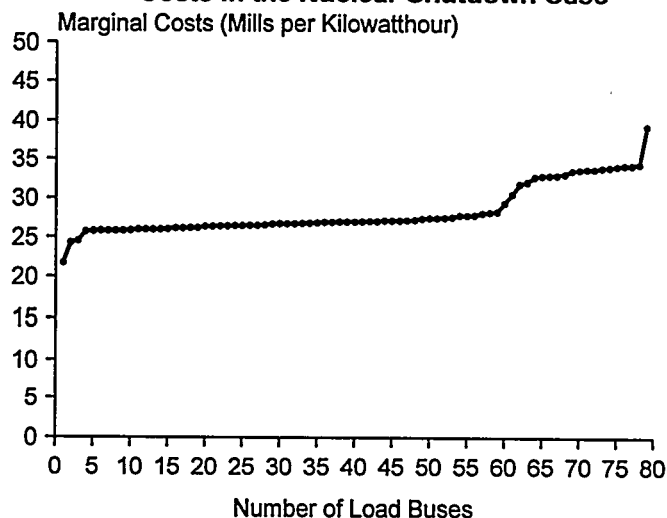
Figure 2. Cumulative Distribution of Short-Run Marginal Generating and Transmission Costs in the Nuclear Shutdown Case
