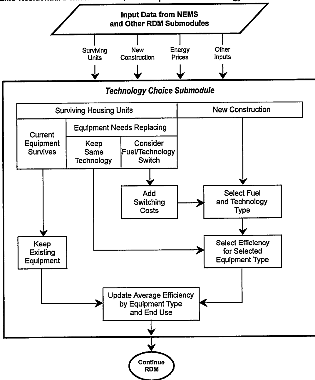
Figure 3. NEMS Residential Demand Module, with Emphasis on Technology Choice
