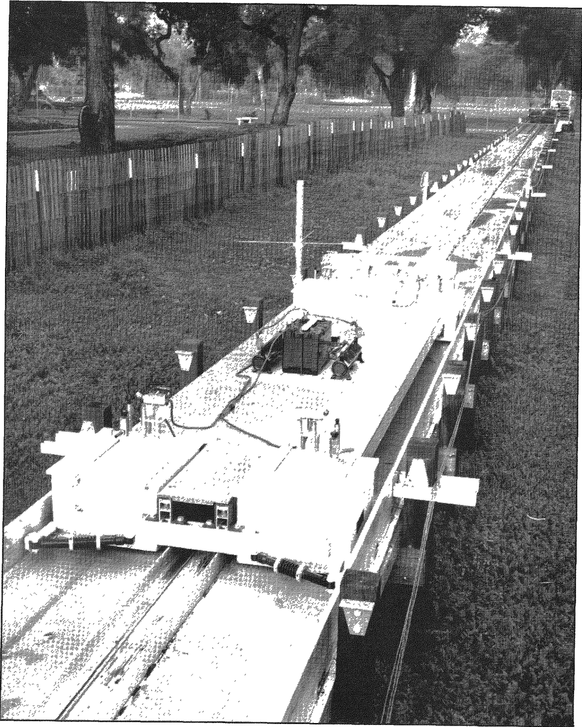
FIGURE B.3 SRI Test "Maglev Vehicle" on U-Shaped Aluminum Guideway (Courtesy SRI International)
