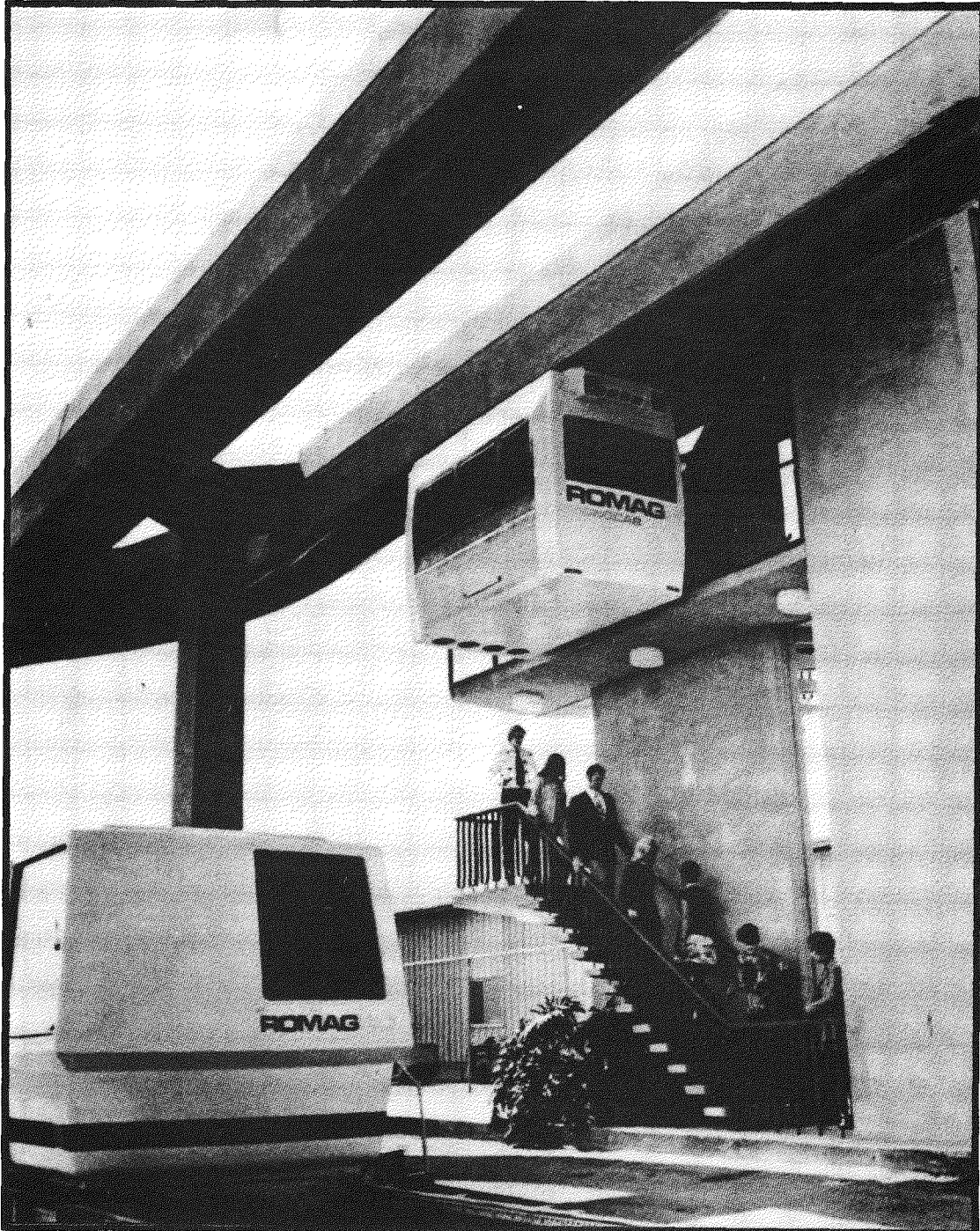
FIGURE B.5 Top-Suspended and Bottom-Supported ROMAG Vehicles at the Rohr Plant in Chula Vista, California (Source: Gilliland, Lytle, and Pearson 1986)
