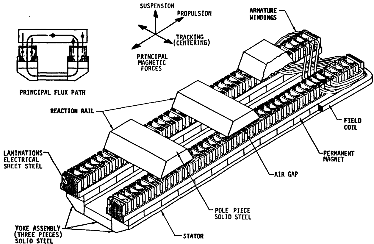
FIGURE B.7 Linear Synchronous Unipolar Motor Developed at Boeing Aerospace (Source: Gilliland, Lyttle, and Pearson 1986)
